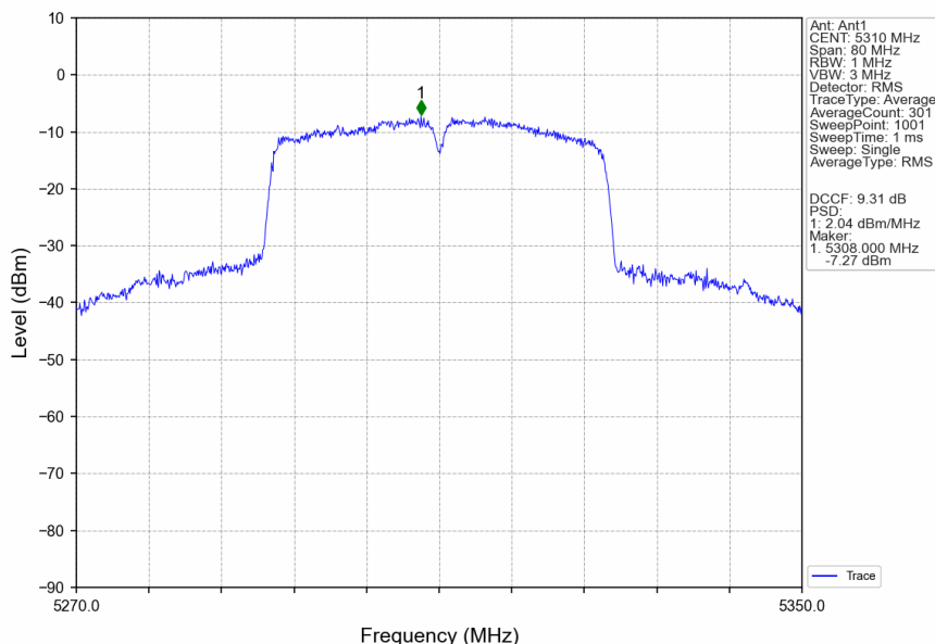
802.11ac(VHT40)_HCH_5310MHz_Ant1_NTNV
