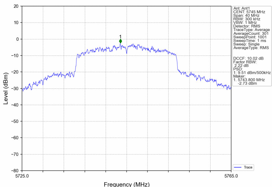
802.11ax(HEW20)_LCH_5745MHz_SU_/_Ant1_NTNV
