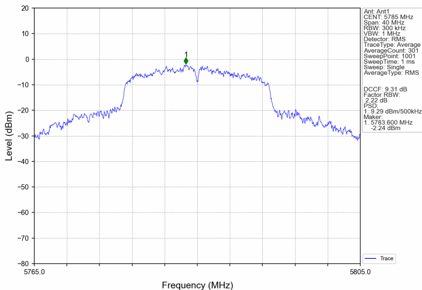
802.11ac(VHT20)_MCH_5785MHz_Ant1_NTNV
