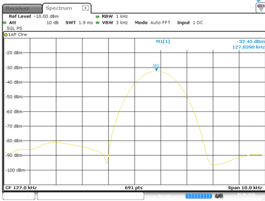
Wireless Charging (Samsung:111-148.5kHz,10W) at +35°C
