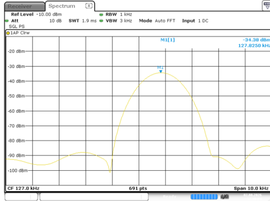
Wireless Charging (Samsung:111-148.5kHz,10W) at +20°C
