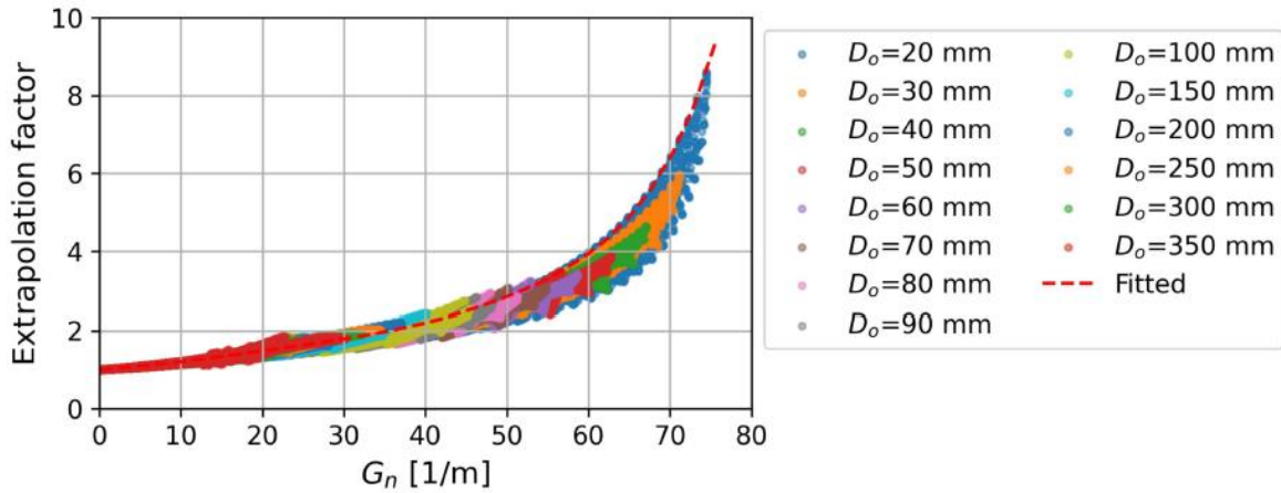
Figure 2.6: Extrapolation factors (i.e., ratios between the simulated results of H_{tip-surface} and \frac{H_{bottom}+H_{top}}{2} ) plotted as a function of the normalized H-field gradient. The data are from simulations of 70 coils with varying outer diameters D_o and filling ratios (0.1–0.9). The predication of the polynomial function \sum_{i=0}^7 c_i [G_n (\Delta d + 11 \text{ mm})]^i with coefficients fitted for the 97.5 th percentile (i.e., the red dashed line) is also shown.
