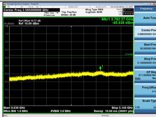
11N20SISO-Ant1-5240-30~5140-PASS
