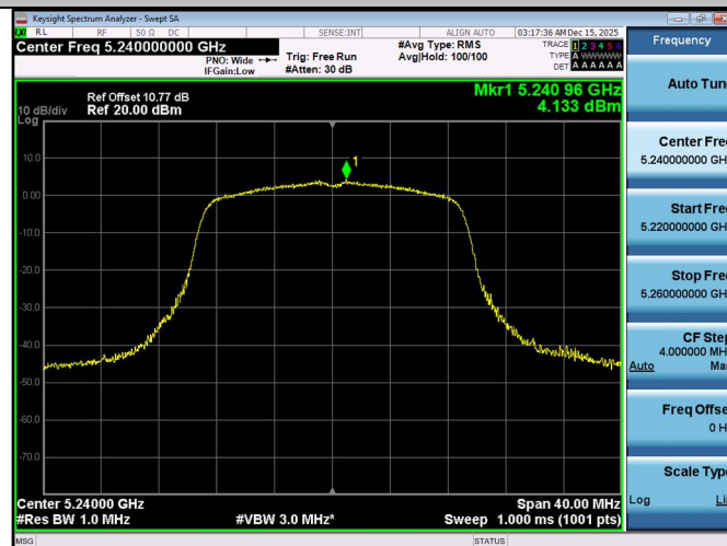
11N20SISO-Ant1-5240-PASS
