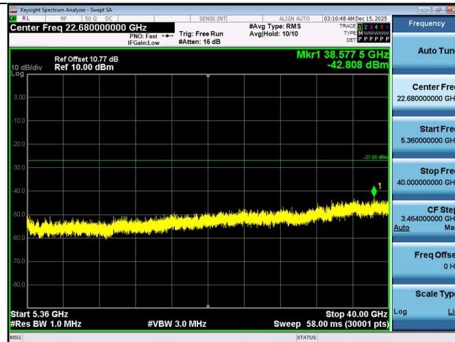
11N20SISO-Ant1-5200-5360~40000-PASS
