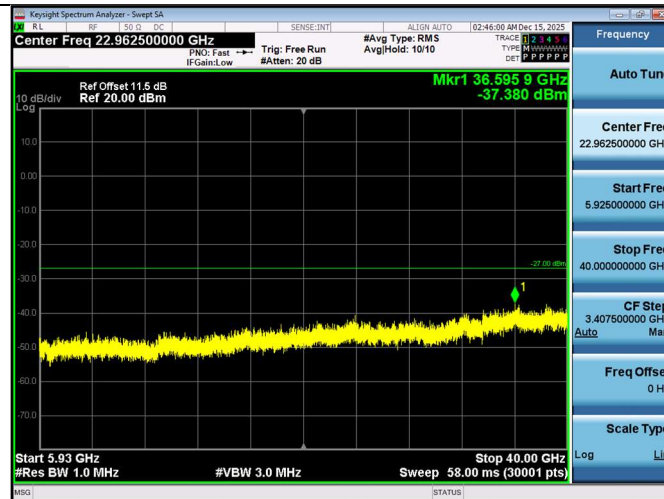
11A-Ant1-5785-5925~40000-PASS
