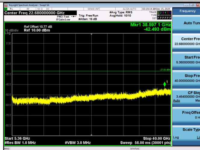
11N20SISO-Ant1-5240-5360~40000-PASS
