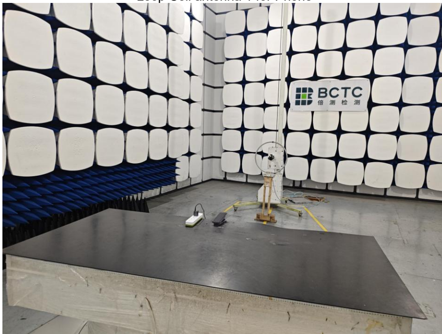
Loop Coil antenna 1 for Phone
