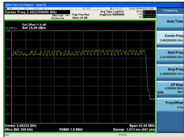
8DPSK 2.4415 GHz ~ 2.4835 GHz
