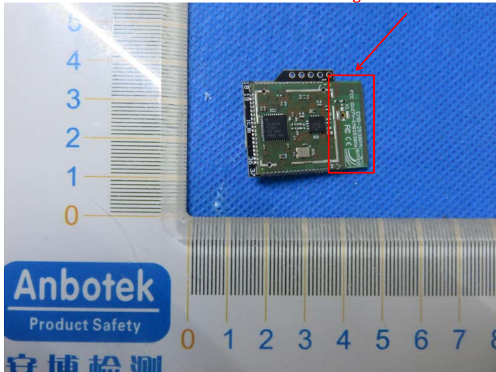
Zigbee Antenna
