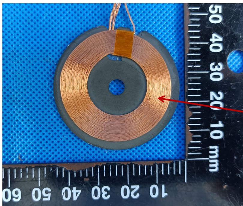
Coil ANT
