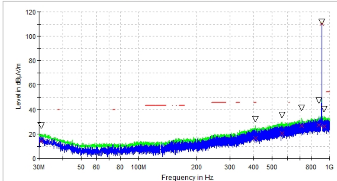
30MHz_1GHz_HP & VP_CH Mid
