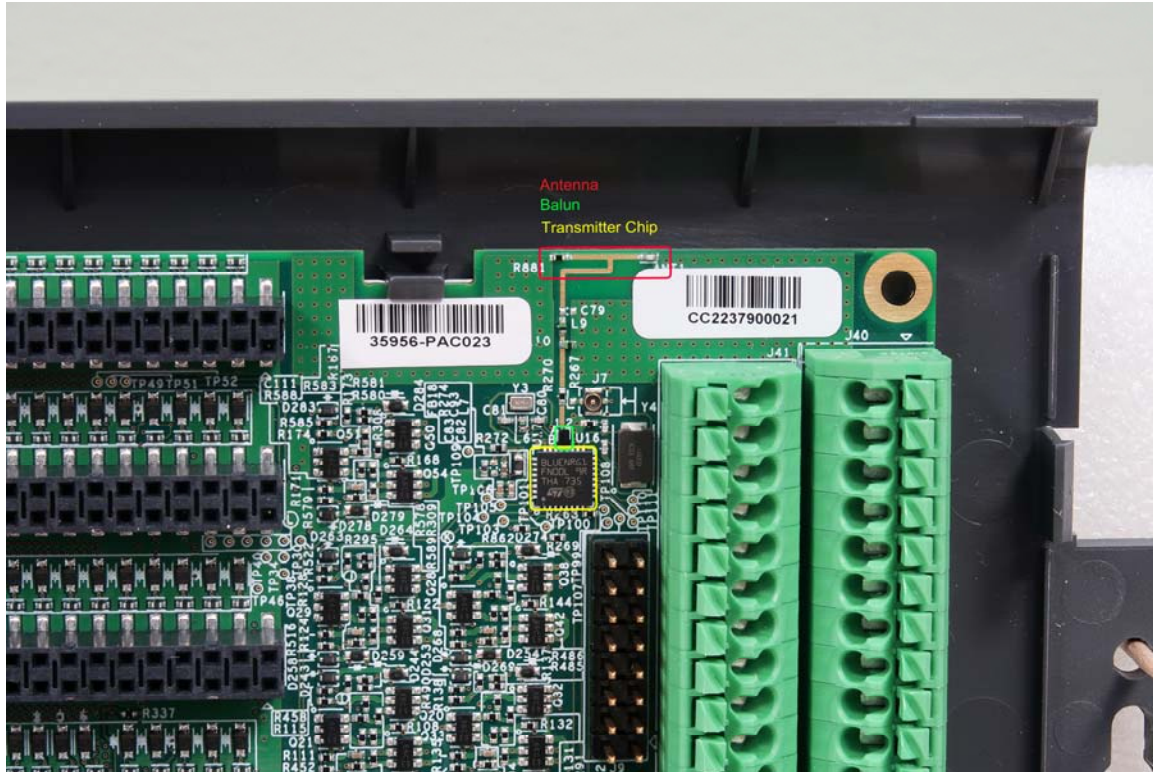
Transmitter and Antenna close Up
