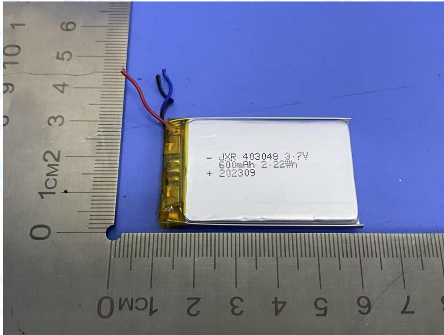
Photo 23 Appearance of Battery
