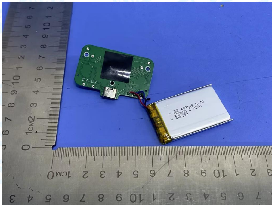
Photo 20 Appearance of PCB & Battery
