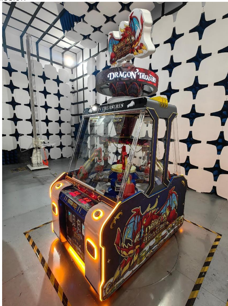
Radiated Emission
