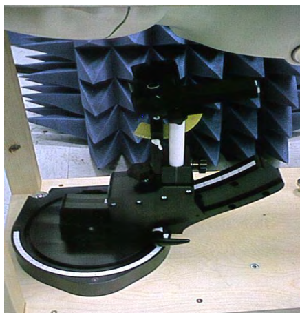
Figure 5. Device Holder
