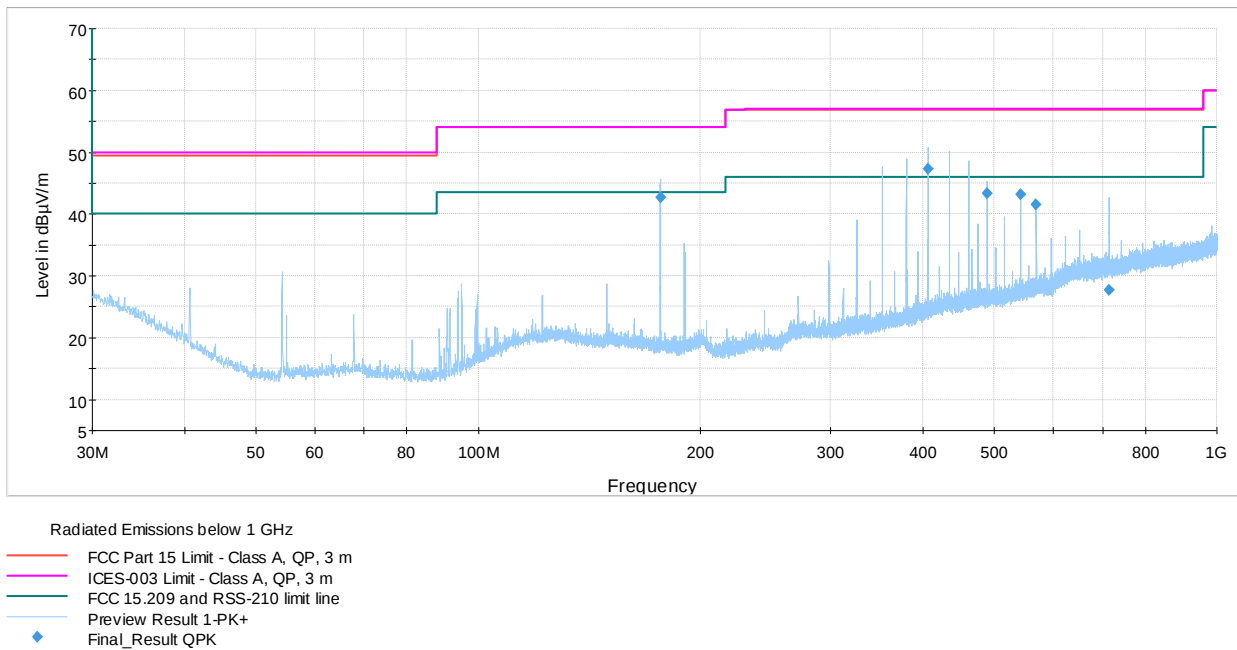
Figure 8.6-2: Field strength of spurious emissions above 30 MHz
