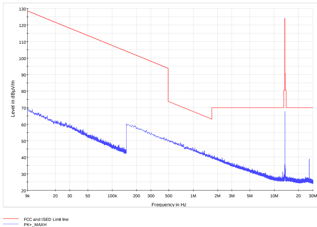
Figure 8.6-1: Field strength of spurious emissions below 30 MHz
