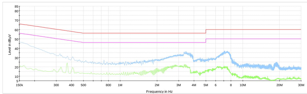
Plot 8.8-3: Conducted emissions on phase line (with loaded antenna)
