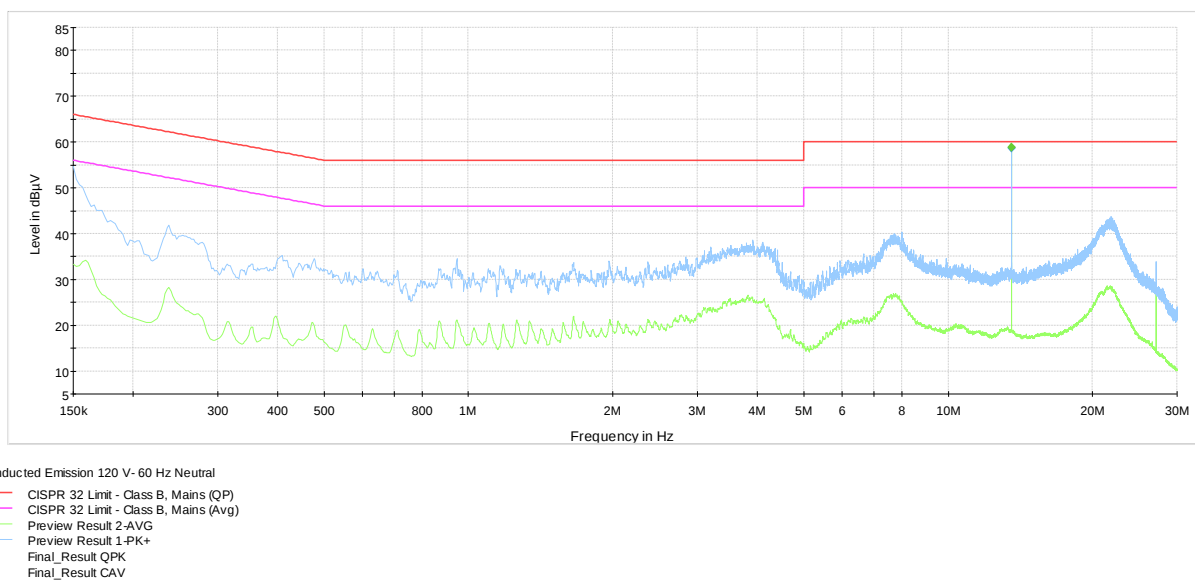
Plot 8.8-2: Conducted emissions on neutral line (without load on antenna)
