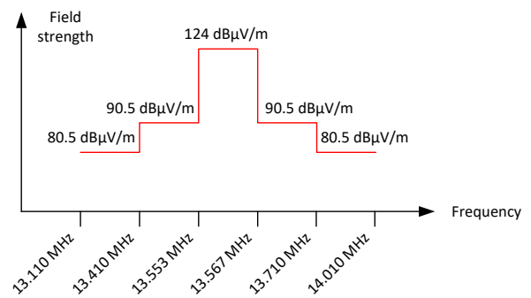
Figure 8.5-2: In-band spurious emissions limit at 3 m
