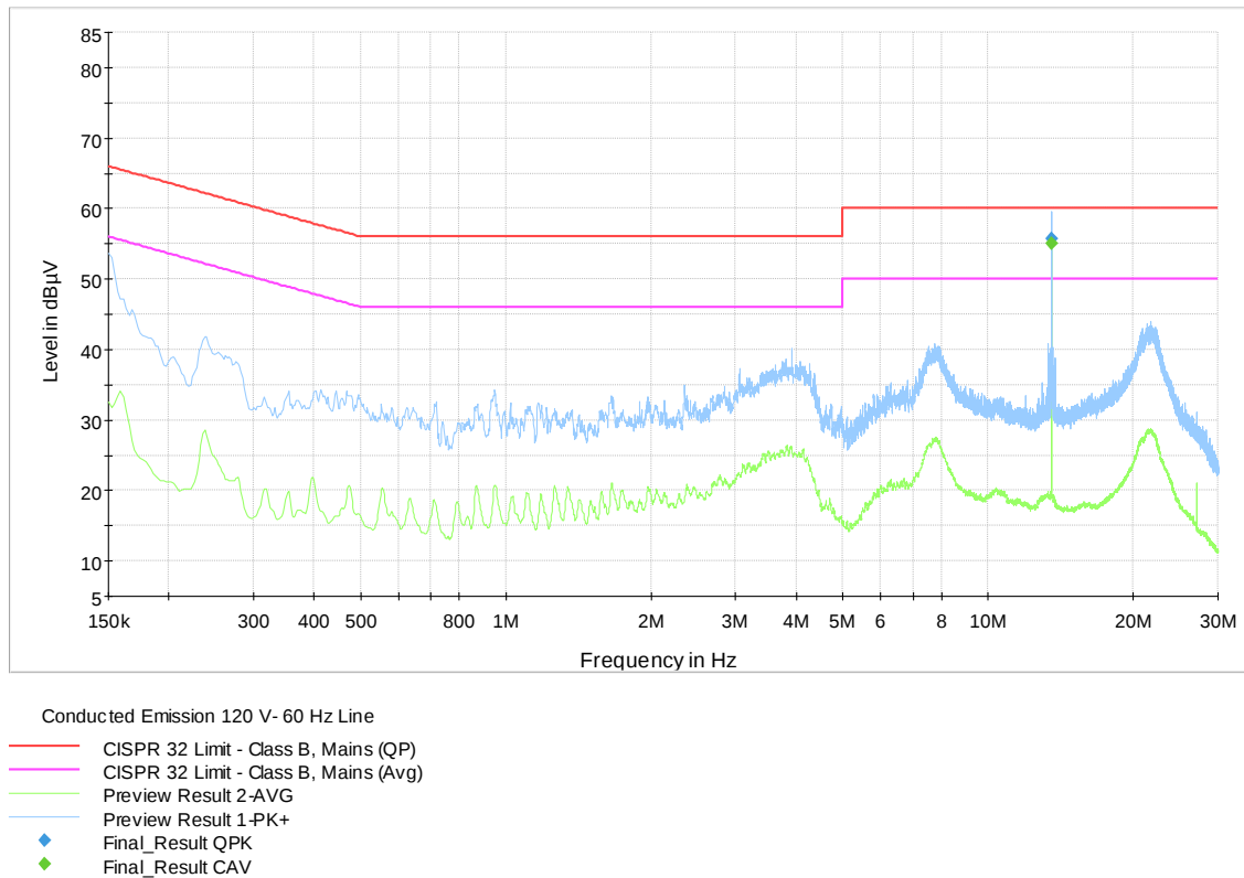
Plot 8.8-1: Conducted emissions on phase line (without load on antenna)
