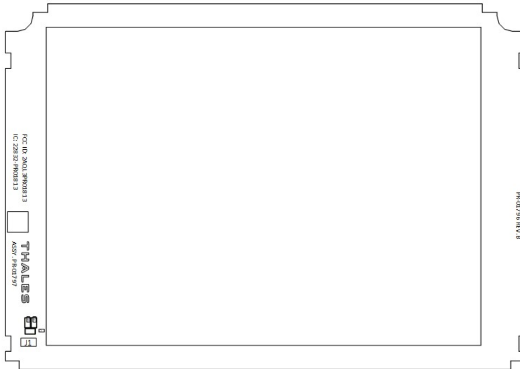
Figure 6. FCC ID/IC marking on PR-01797 glass antenna.
