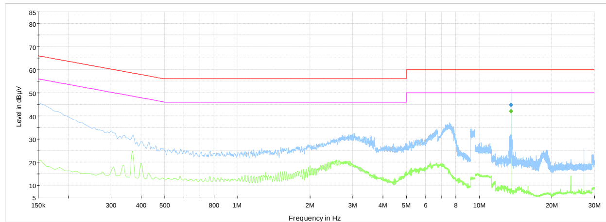
Plot 8.8-3: Conducted emissions on phase line (with loaded antenna)
