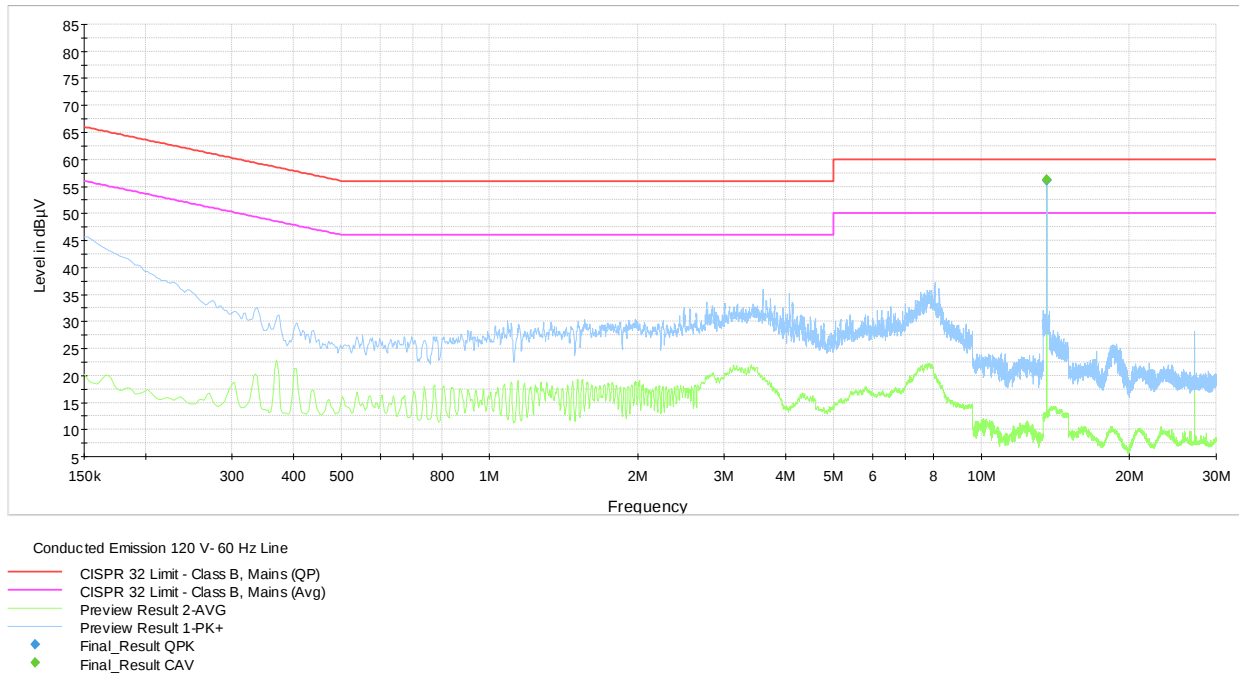
Plot 8.8-1: Conducted emissions on phase line (without load on antenna)
