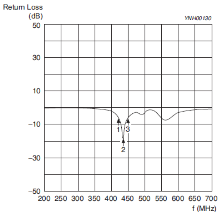
Return loss
