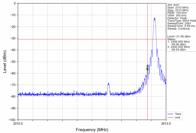
Zigbee_LCH_2405MHz_Ant1_NTNV
