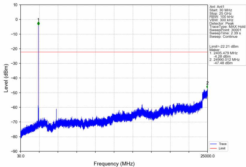
Zigbee_LCH_2405MHz_Ant1_NTNV
