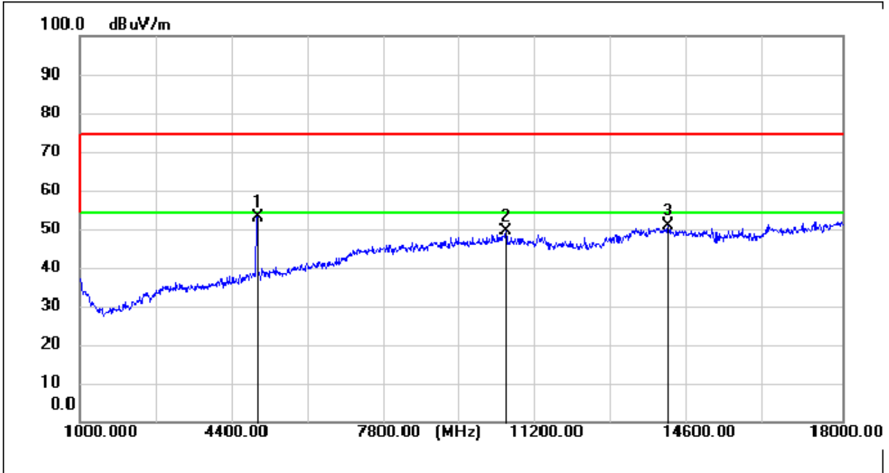
Zigbee_TX_CH_2480_Vertical
