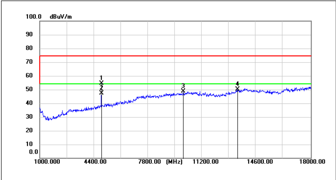
Zigbee_TX_CH_2440_Vertical
