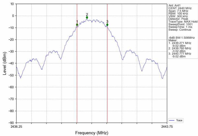
Zigbee_MCH_2440MHz_Ant1_NTNV
