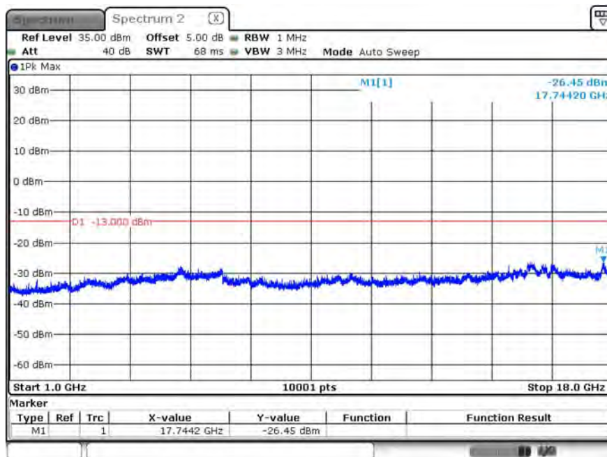
B26_CH26705_3M_1RB0_16-QAM_Above 1G
