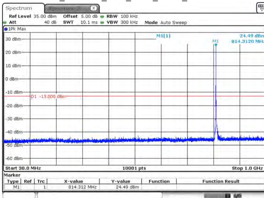
B26_CH26697_1.4M_1RB0_QPSK_Below 1G
