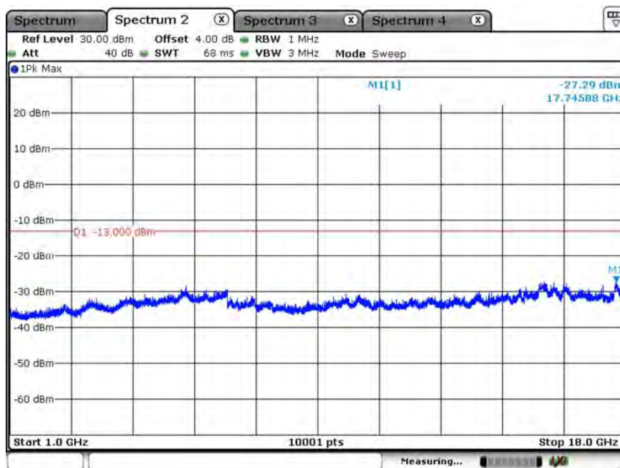
B71_CH113147_5M_1RB0_QPSK_Above 1G
