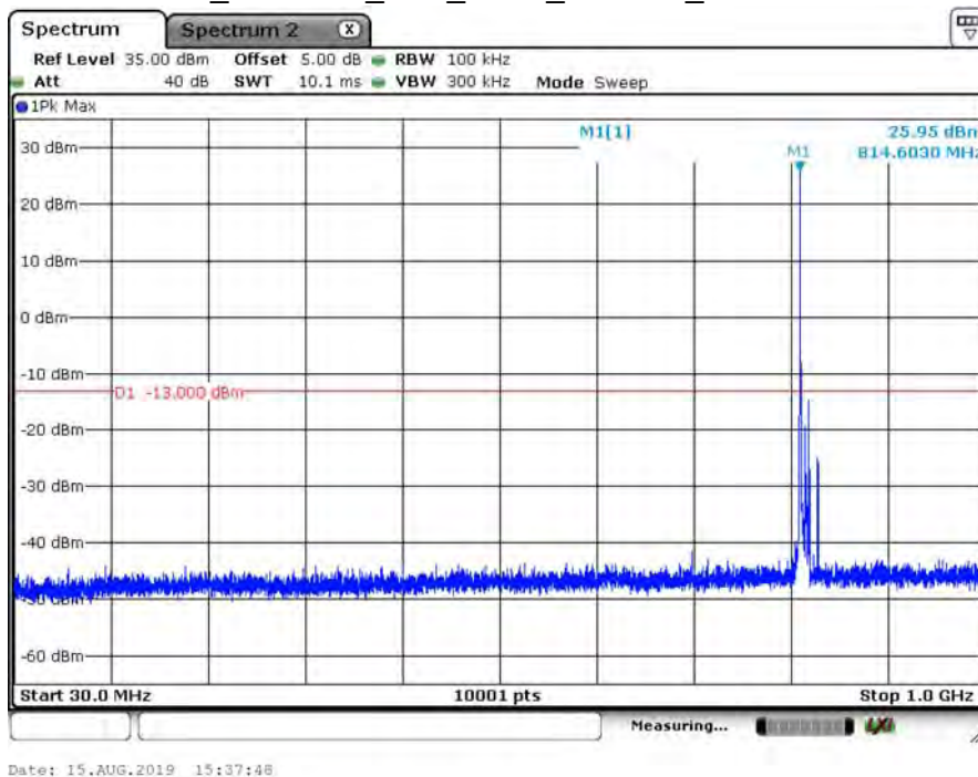
B26_CH26740_10M_1RB0_16-QAM_Below 1G
