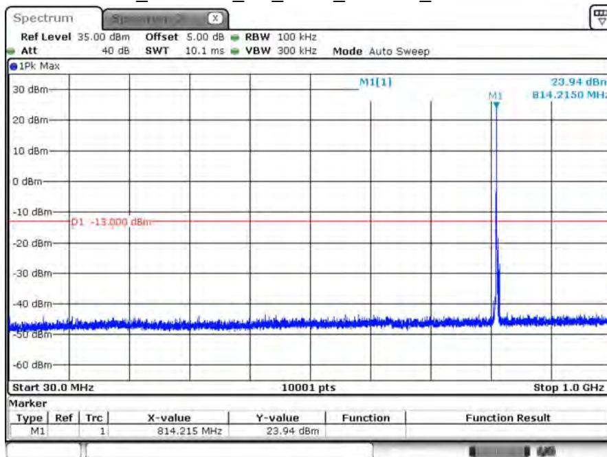
B26_CH26705_3M_1RB0_16-QAM_Below 1G
