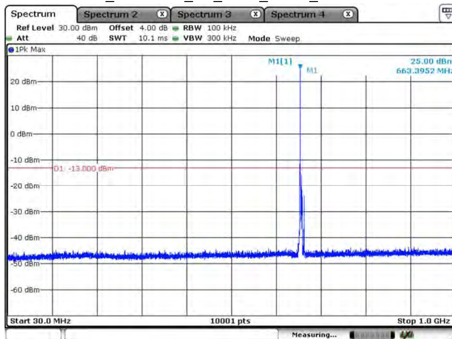
B71_CH113147_5M_1RB0_QPSK_Below 1G
