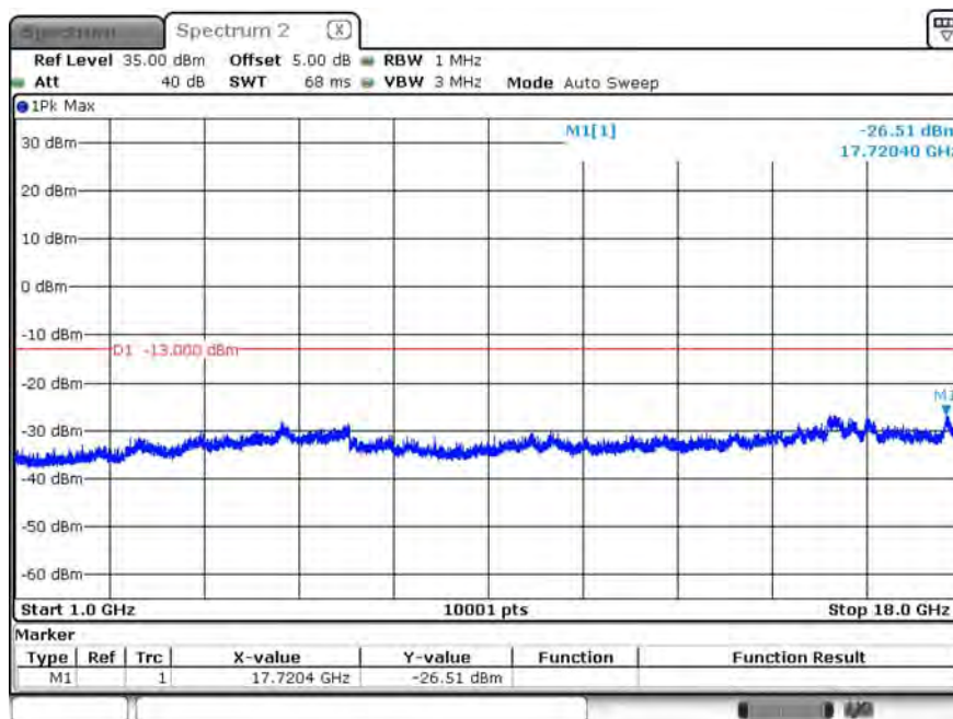
B26_CH26697_1.4M_1RB0_QPSK_Above 1G
