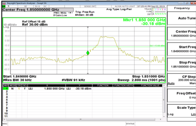
Cat_M1_Band2_1_4MHz_QPSK_1_0_LowCH18607-1850.7
