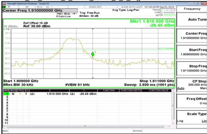
Cat_M1_Band2_1_4MHz_QPSK_1_5_HighCH19193-1909.3
