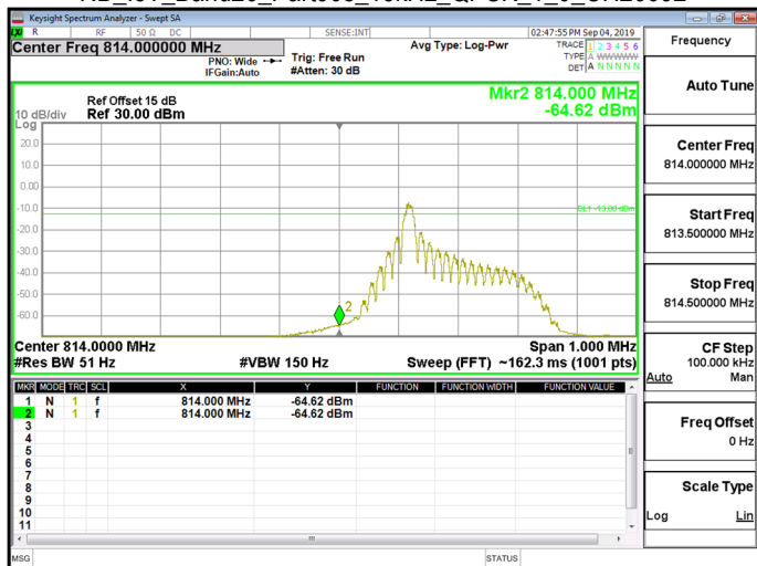
NB_IoT_Band26_Part90s_15kHz_QPSK_1_11_CH26788
