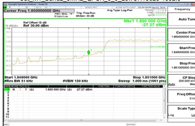
Cat_M1_Band2_5MHz_QPSK_6_0_LowCH18625-1852.5
