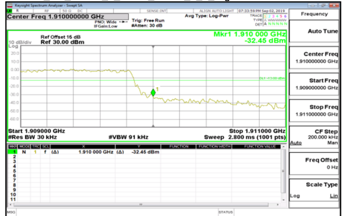
Cat_M1_Band2_1_4MHz_QPSK_6_0_HighCH19193-1909.3
