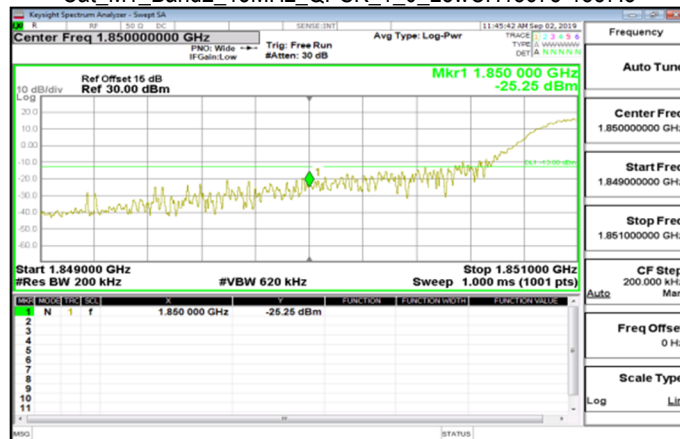
Cat_M1_Band2_15MHz_QPSK_1_0_LowCH18675-1857.5
