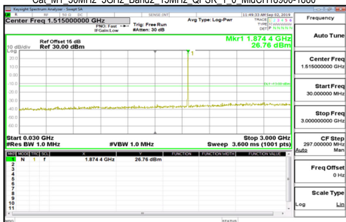
Cat_M1_30MHz~3GHz_Band2_15MHz_QPSK_1_0_MidCH18900-1880
