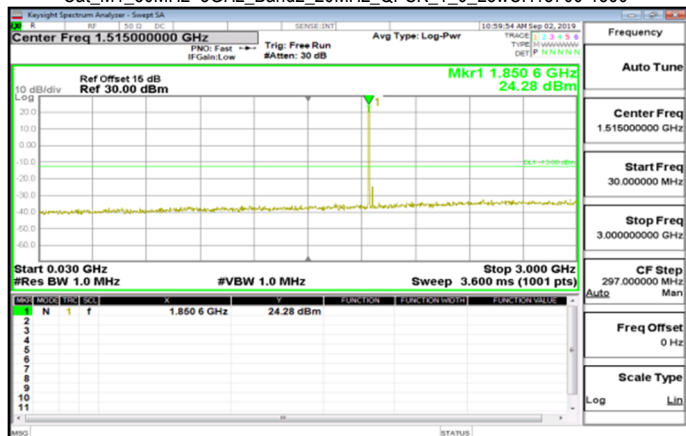
Cat M1_30MHz~3GHz_Band2_20MHz_QPSK_1_0_LowCH18700-1860
