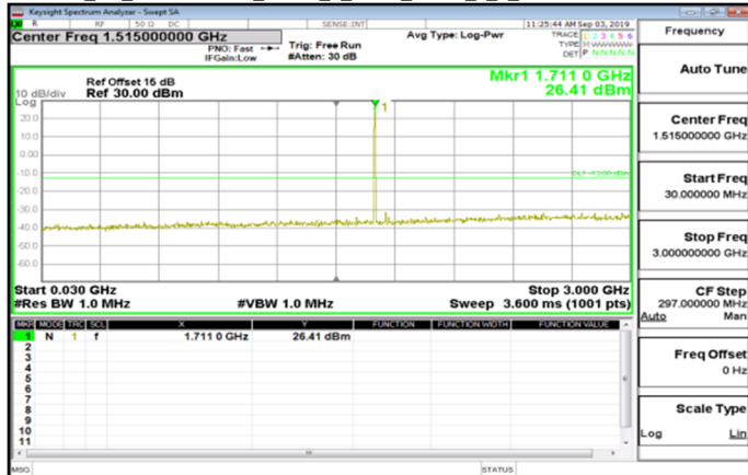
Cat M1_30MHz~3GHz_Band4_1_4MHz_QPSK_1_0_LowCH19957-1710.7
