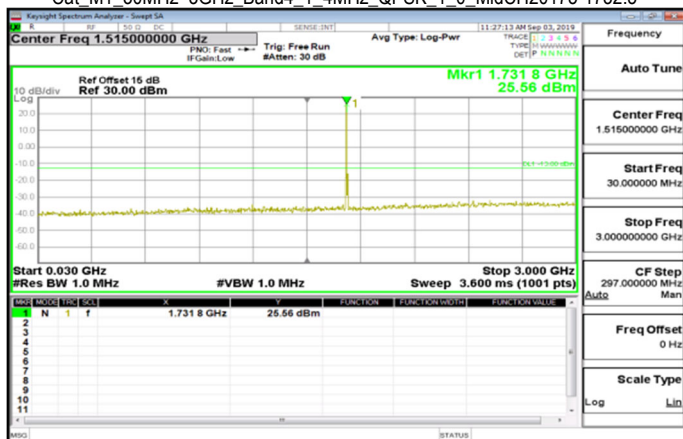
Cat M1_30MHz~3GHz_Band4_1_4MHz_QPSK_1_0_MidCH20175-1732.5
