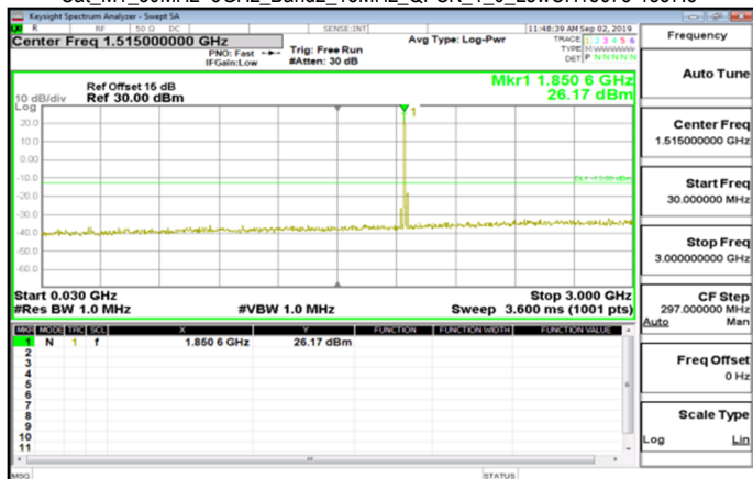
Cat_M1_30MHz~3GHz_Band2_15MHz_QPSK_1_0_LowCH18675-1857.5
