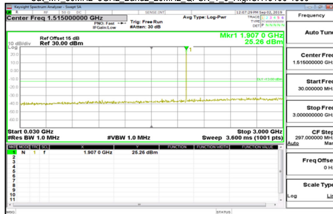
Cat M1_30MHz~3GHz_Band2_20MHz_QPSK_1_0_HighCH19100-1900
