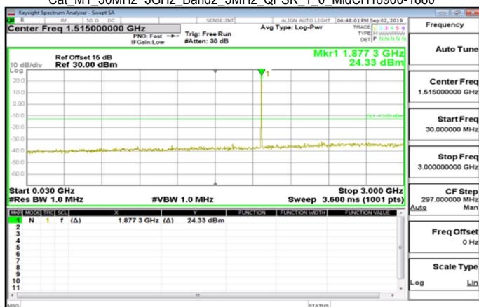
Cat_M1_30MHz~3GHz_Band2_5MHz_QPSK_1_0_MidCH18900-1880
