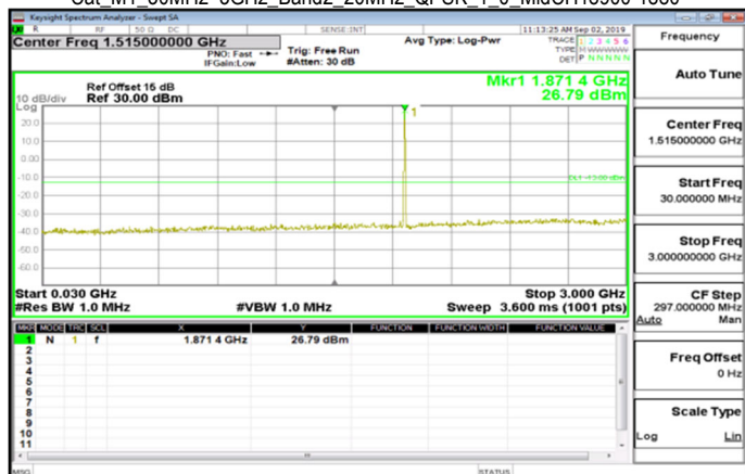
Cat M1_30MHz~3GHz_Band2_20MHz_QPSK_1_0_MidCH18900-1880
