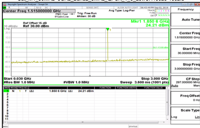
Cat_M1_30MHz~3GHz_Band2_5MHz_QPSK_1_0_LowCH18625-1882.5
