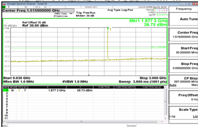
Cat M1_30MHz~3GHz_Band2_10MHz_QPSK_1_0_MidCH18900-1880
