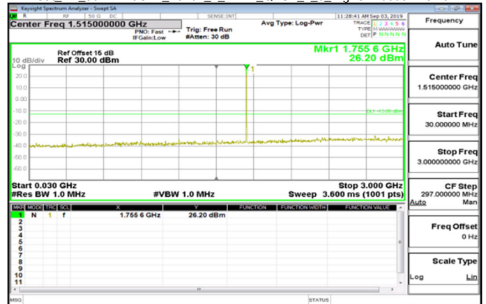
Cat M1_30MHz~3GHz_Band4_1_4MHz_QPSK_1_0_HighCH20393-1754.3
