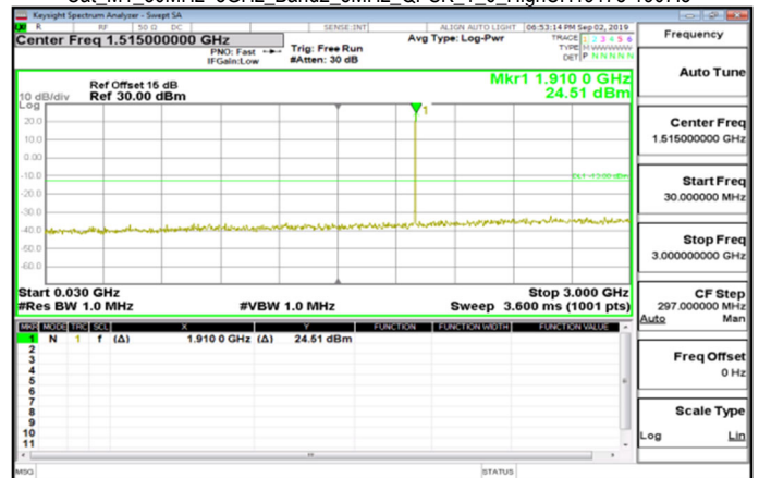
Cat_M1_30MHz~3GHz_Band2_5MHz_QPSK_1_0_HighCH19175-1907.5
