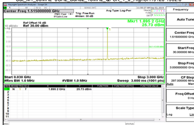
Cat_M1_30MHz~3GHz_Band2_15MHz_QPSK_1_0_HighCH19125-1902.5
