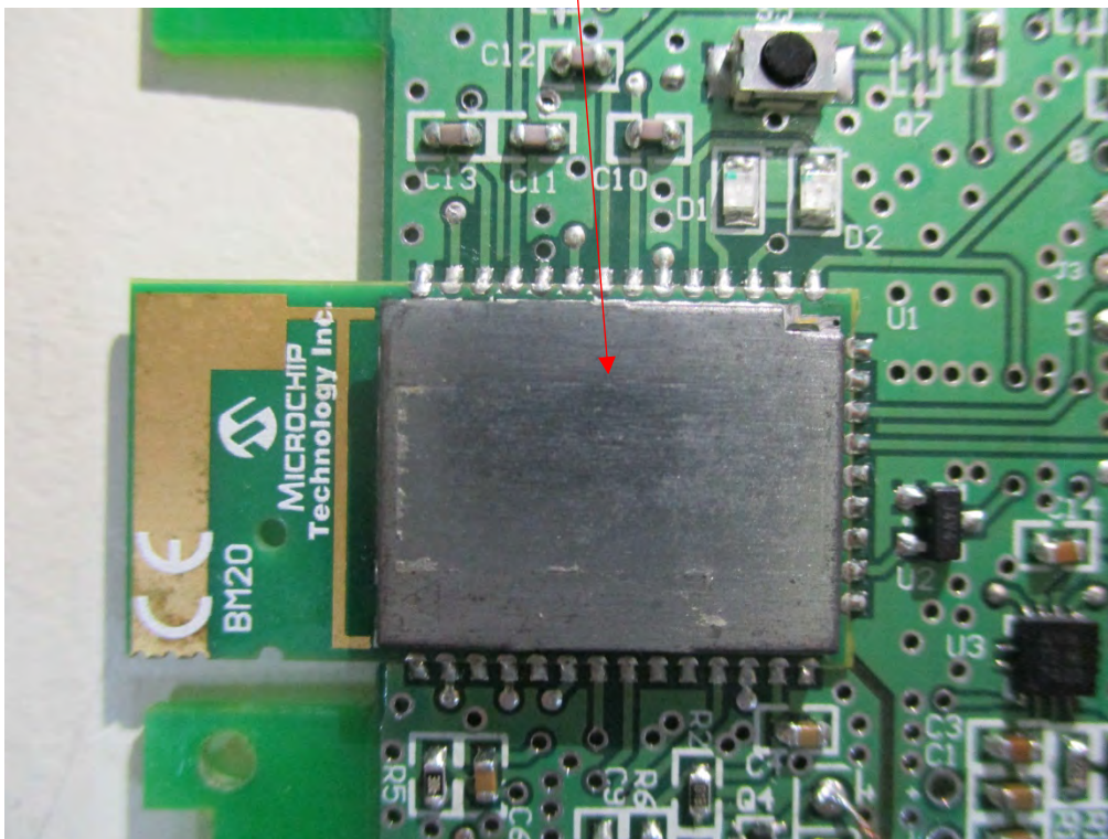
RF Module – Top View
