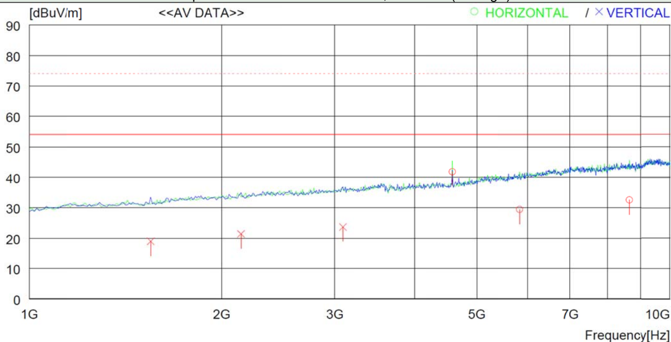
Tabulated Test Data – Above 1 GHz, Channel2 (Average)
