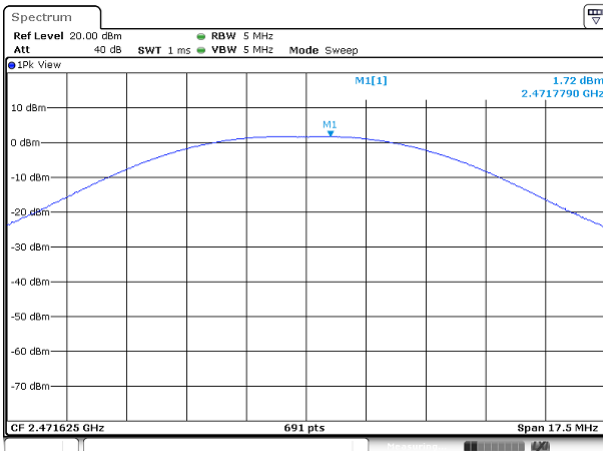
Peak output Power plot on channel 20 (1Mbps)
