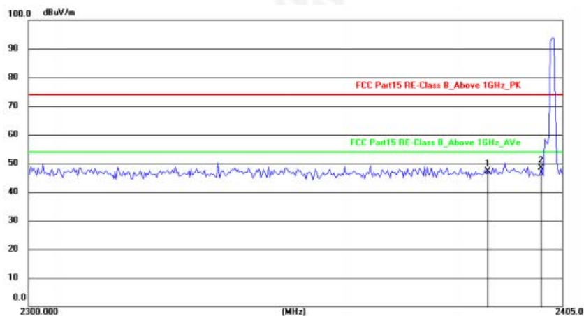
2402MHz Horizontal
