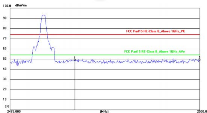
2480MHz Vertical
