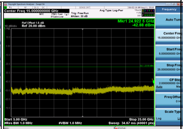
802.11g,2462MHz,Ant1,Plot 5,5000MHz~25000MHz
