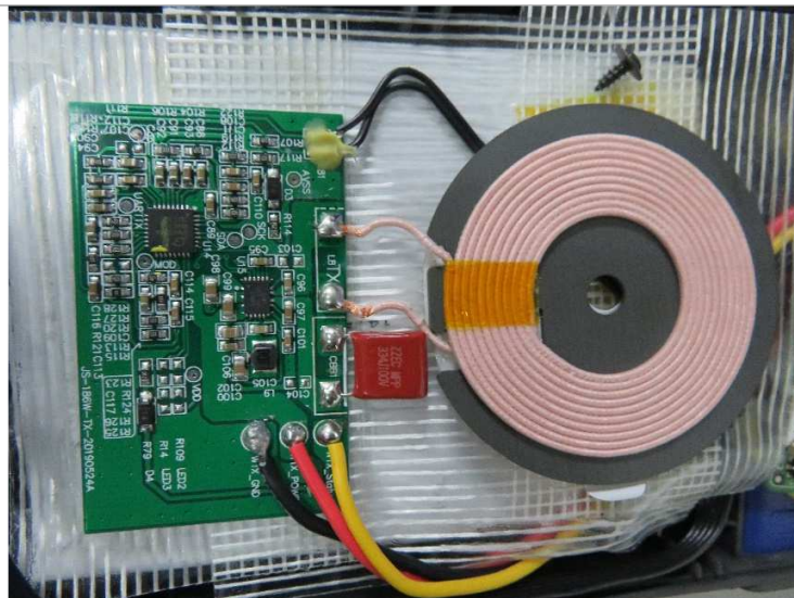
PCB and coil view
