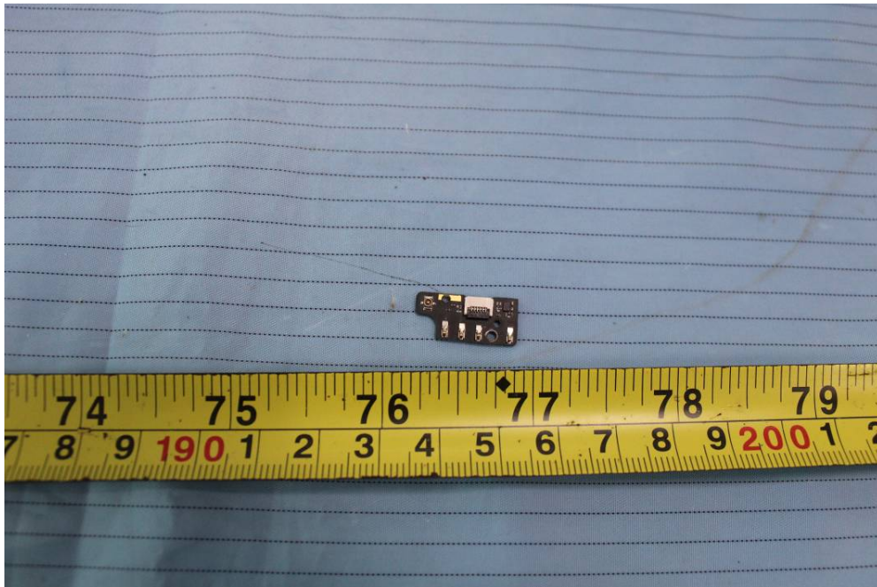
EUT – Small Main Board Top View
