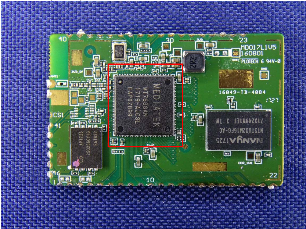
(19) EUT Photo (Module)
