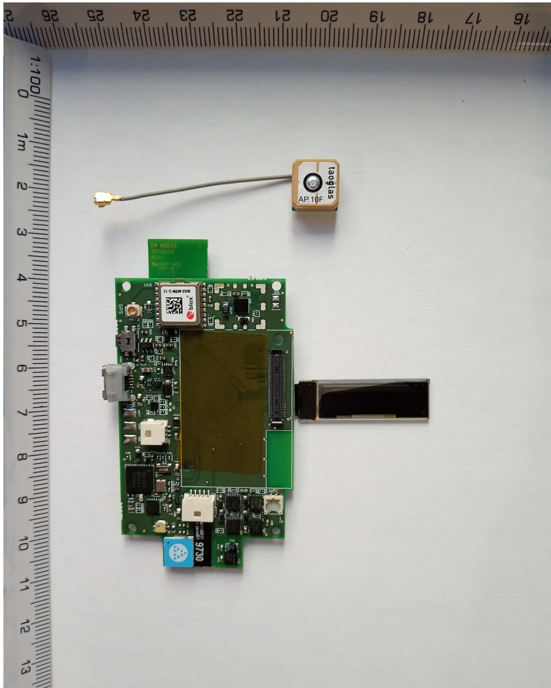
Photo 3: WIMU PRO – PCB side 1 and GNSS antenna.
