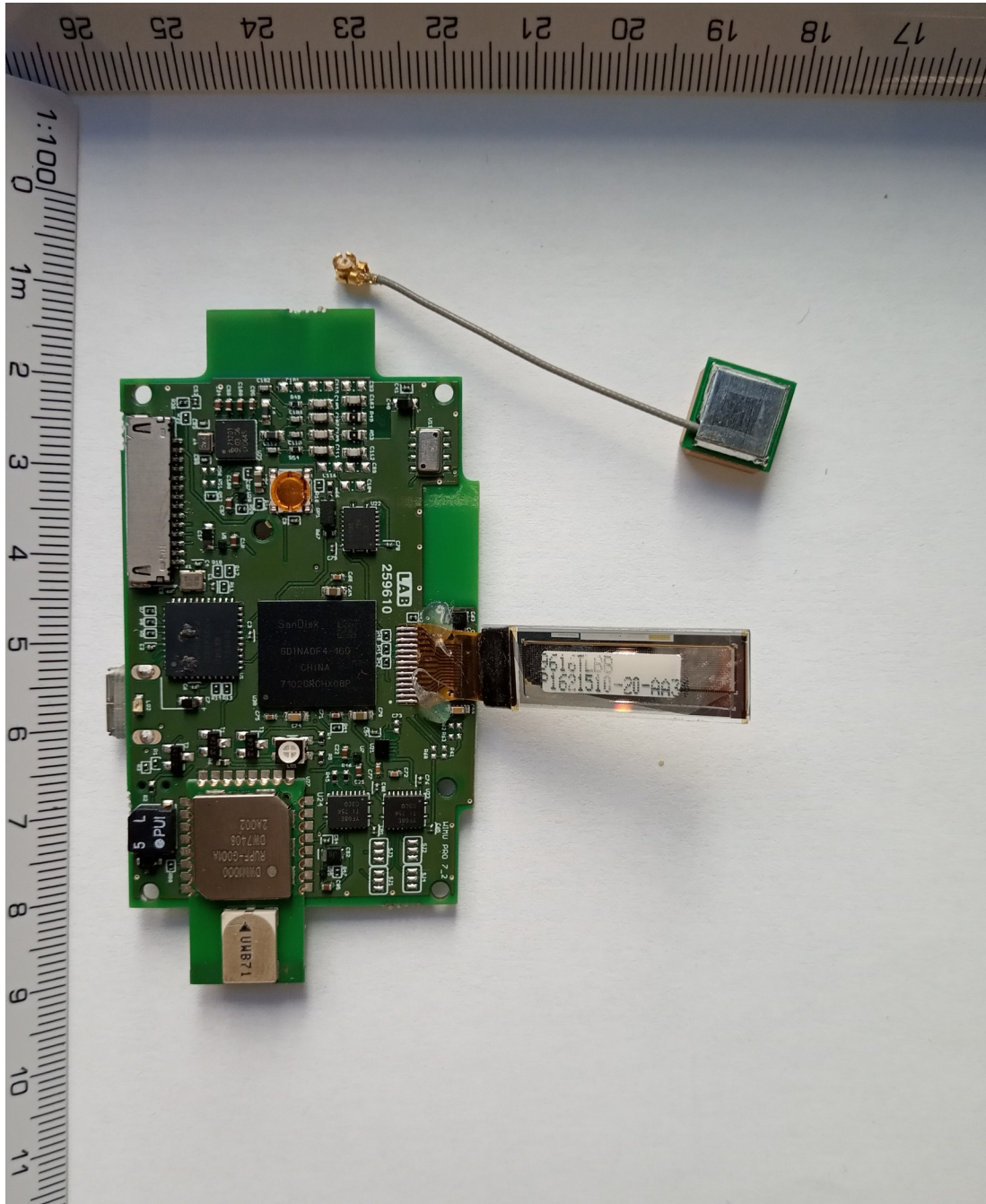
Photo 4: WIMU PRO – PCB side 2 and GNSS antenna.
