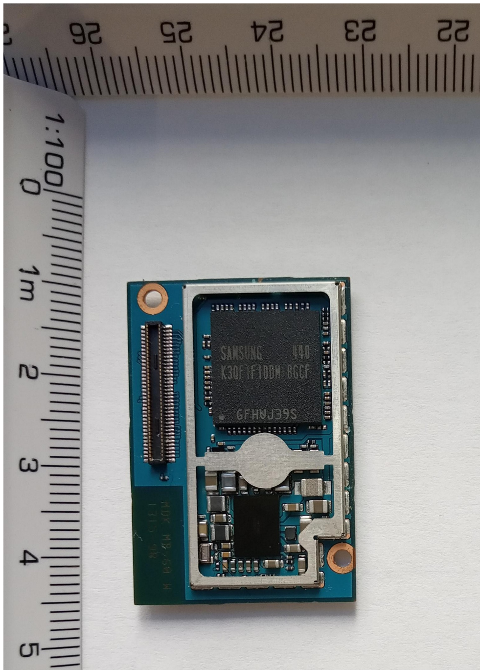
Photo 6: WIMU PRO – Edison without shield, side 2.
