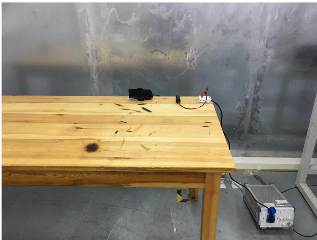
Conducted Emission
