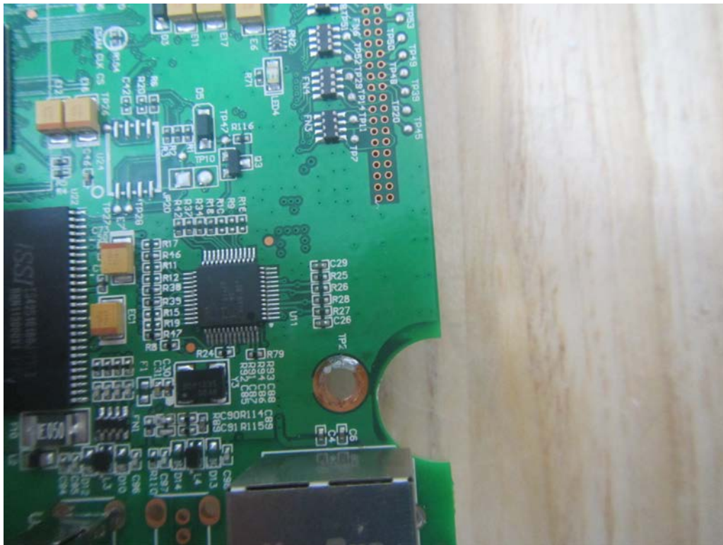
Detail View of EUT-16
