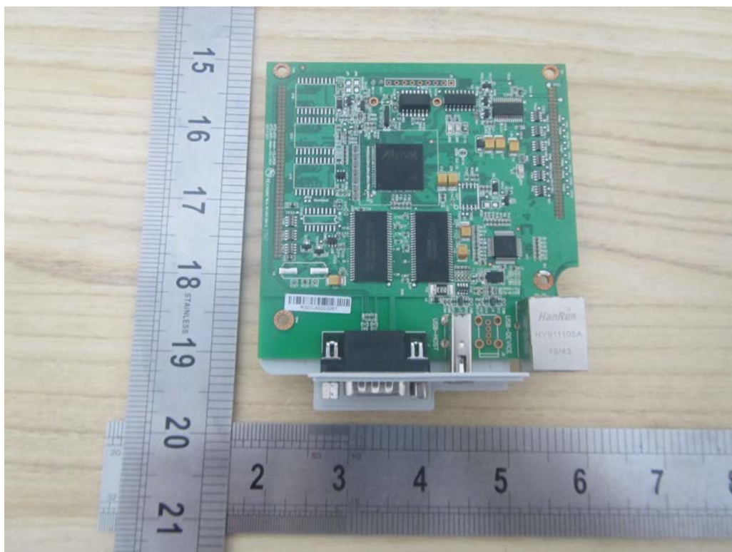
Detail View of EUT-13
