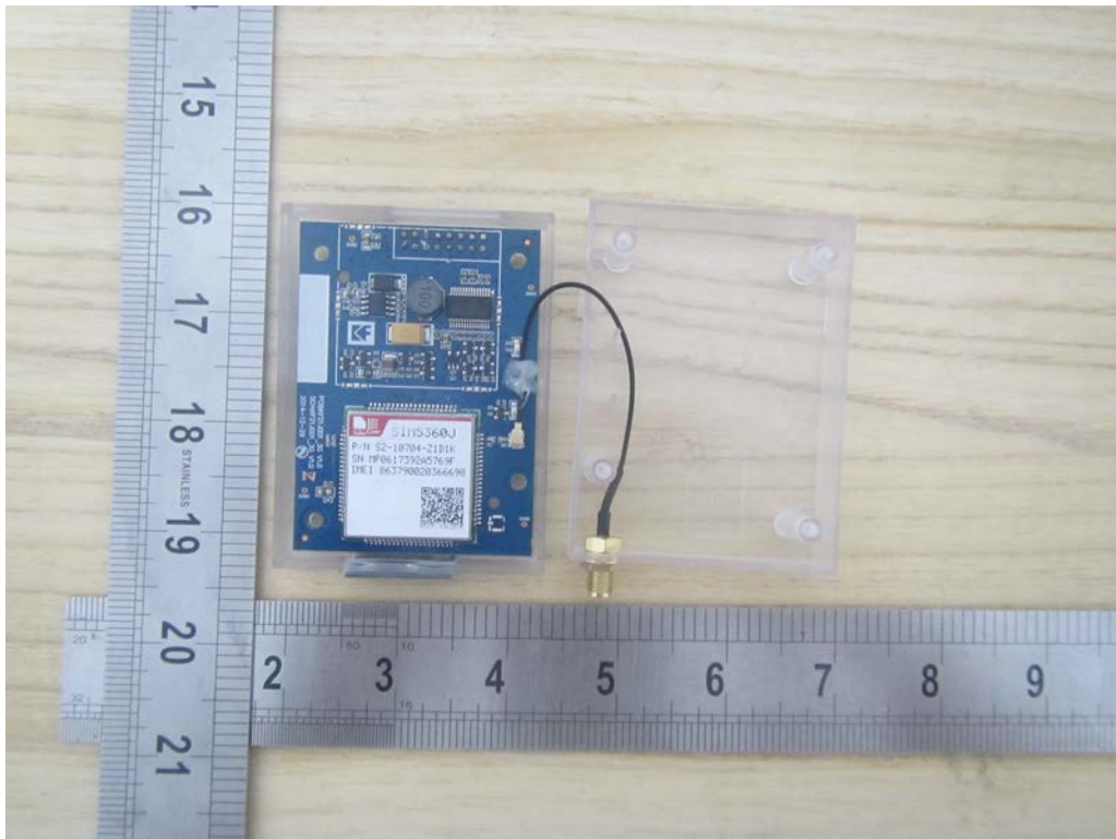
Detail View of EUT-5
