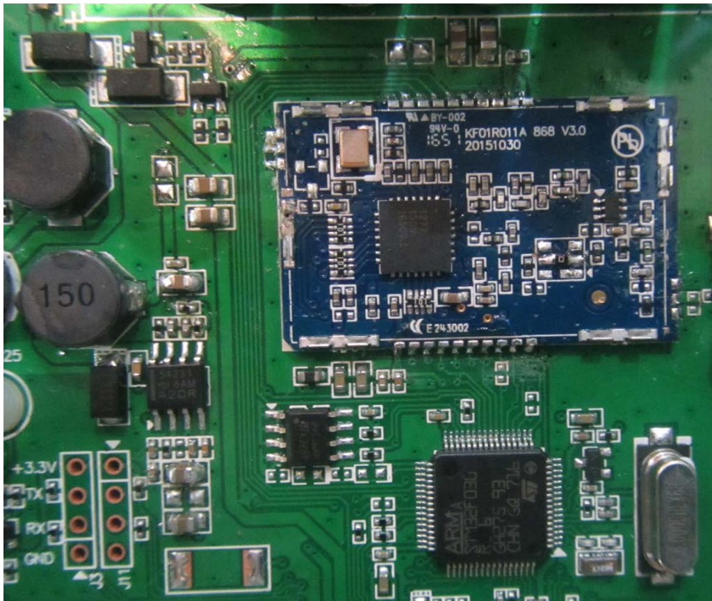
Detail View of EUT-24
