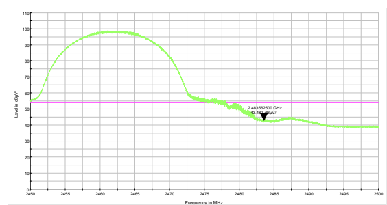
802.11b-Channel 11 Average
