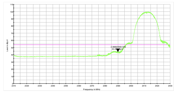
802.11b-Channel 1 Average
