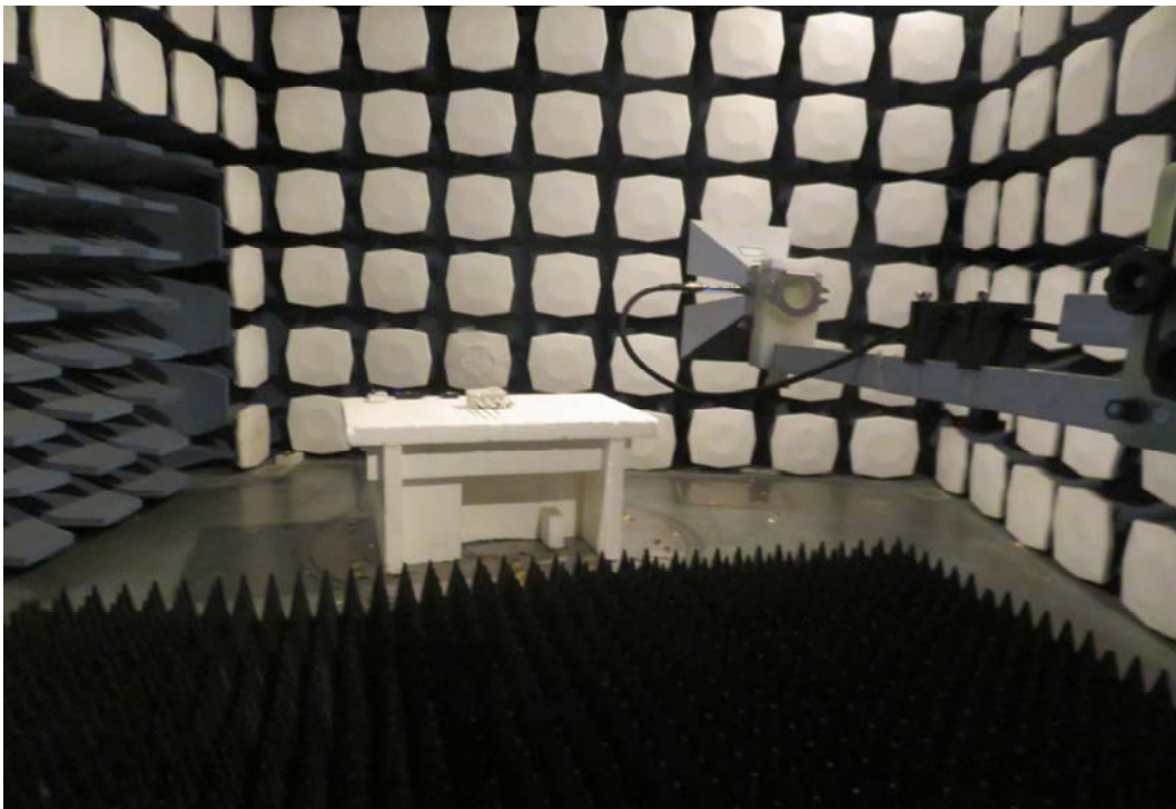
Picture : Radiated Spurious Emissions Test setup
