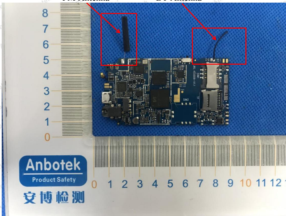
FM Antenna
