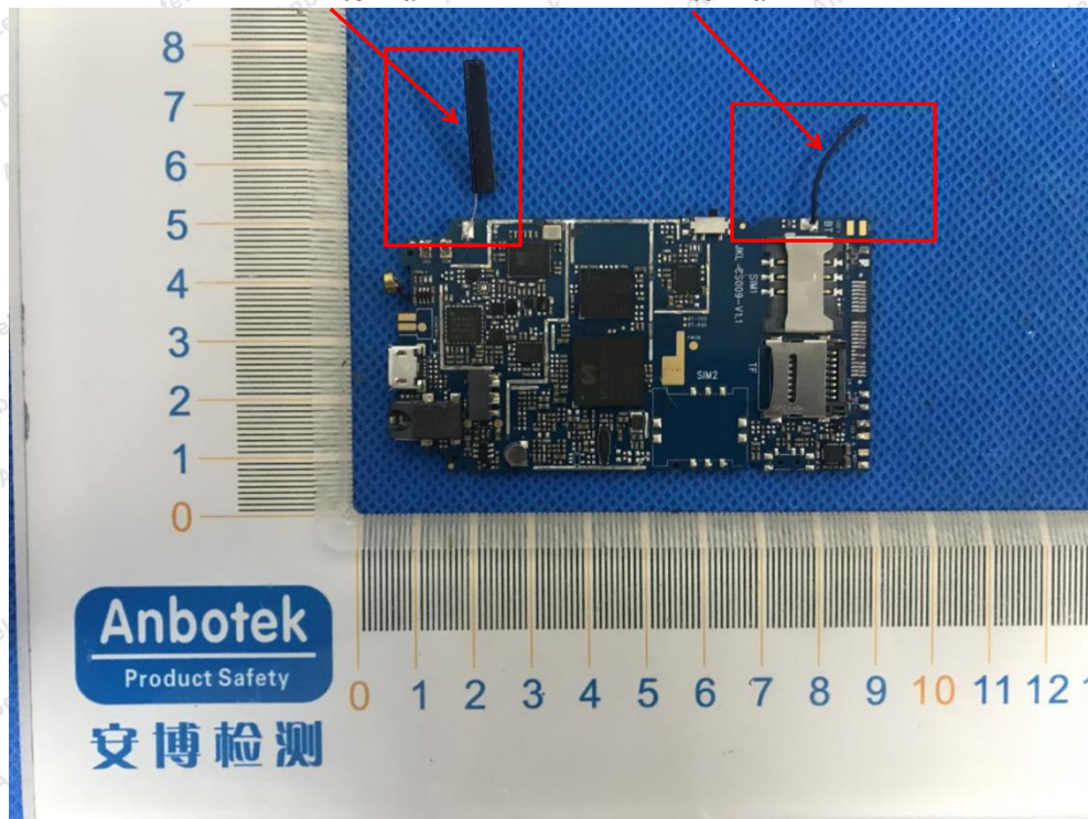
FM Antenna
