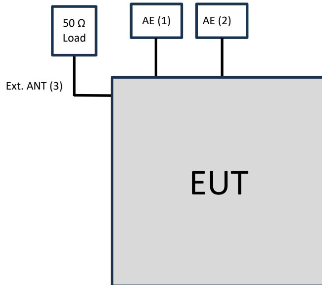
EUT connection diagram for configuration #1
