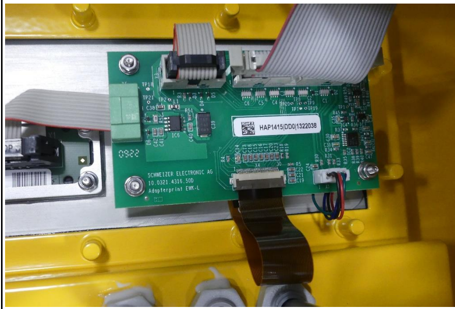
Display/Keyboard PCB top view
