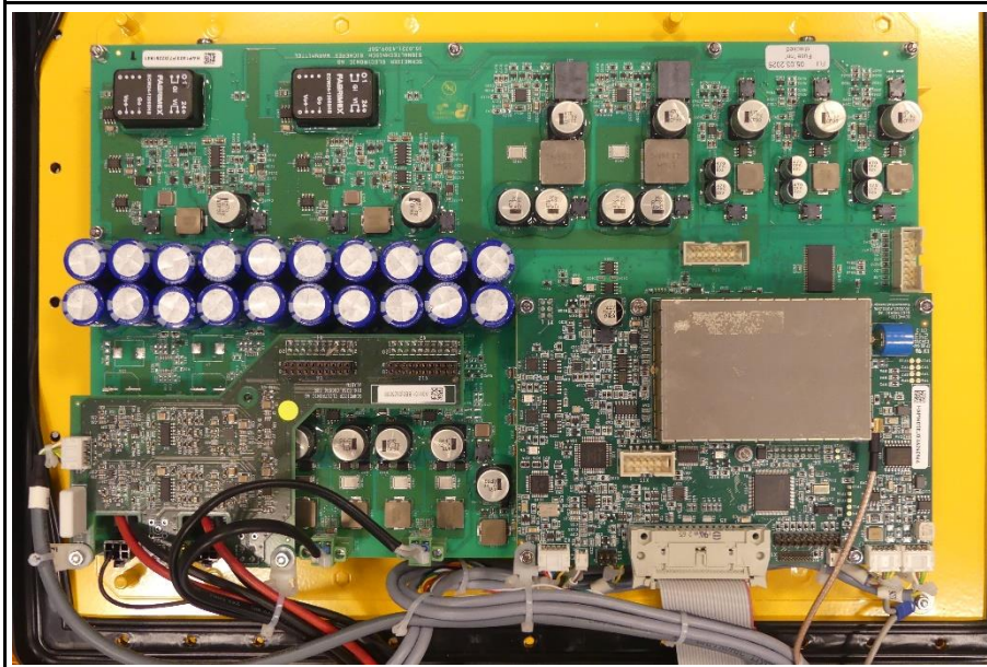
PCB2 top side
