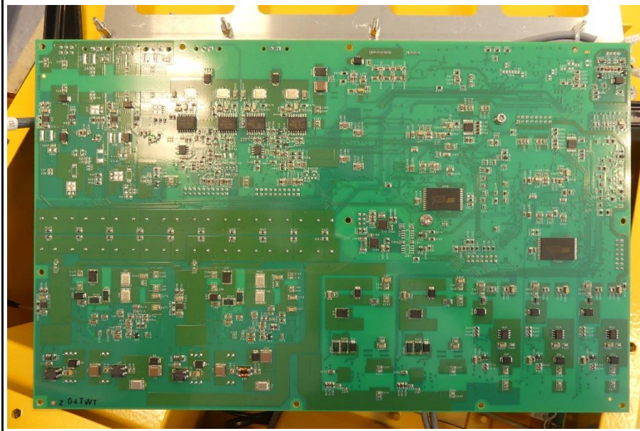
PCB2 bottom side
