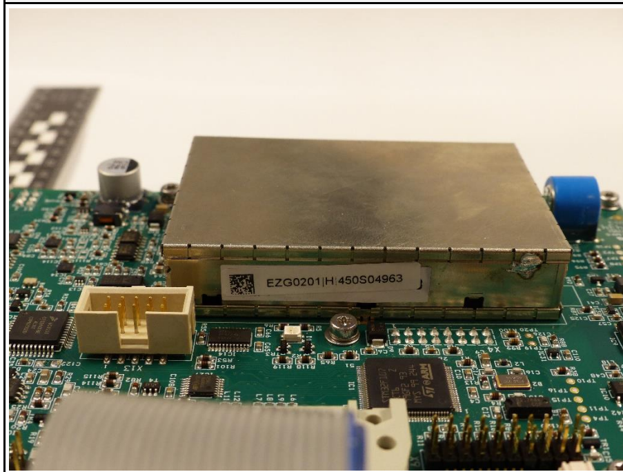
Radio unit with label and shielding
