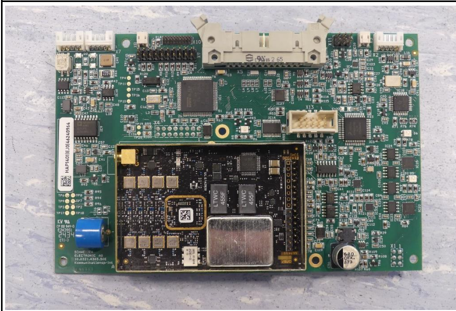
Radio PCB top view
