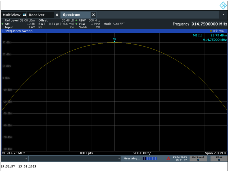
Figure 21 - 914.75
