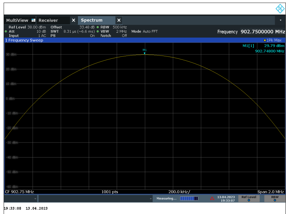
Figure 20 - 902.75
