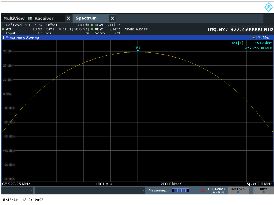
Figure 25 - 927.25
