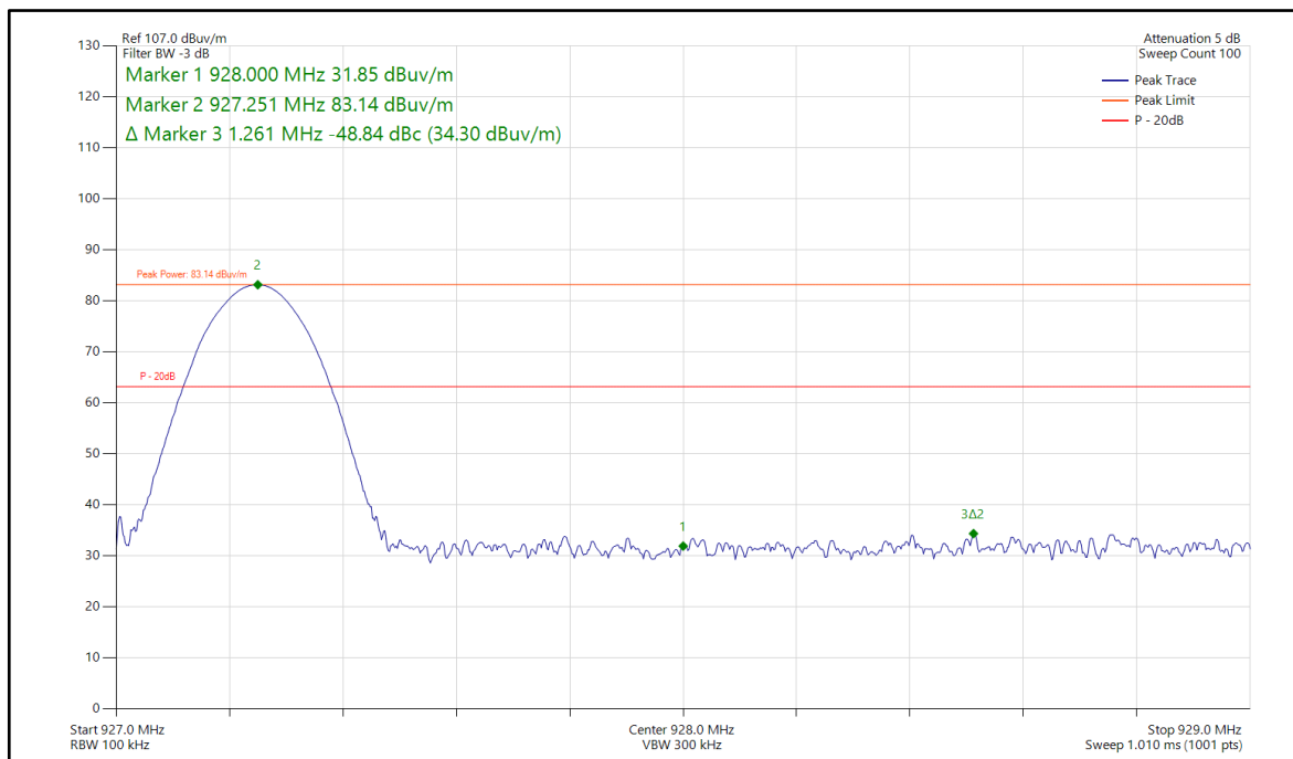
Figure 29 - FHSS, 927.25MHz, Band Edge Frequency 928 MHz
