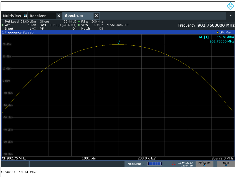
Figure 23 - 902.75
