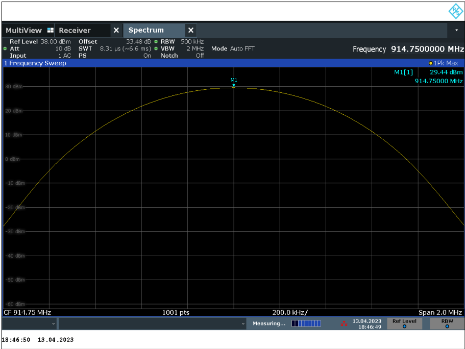
Figure 24 - 914.75
