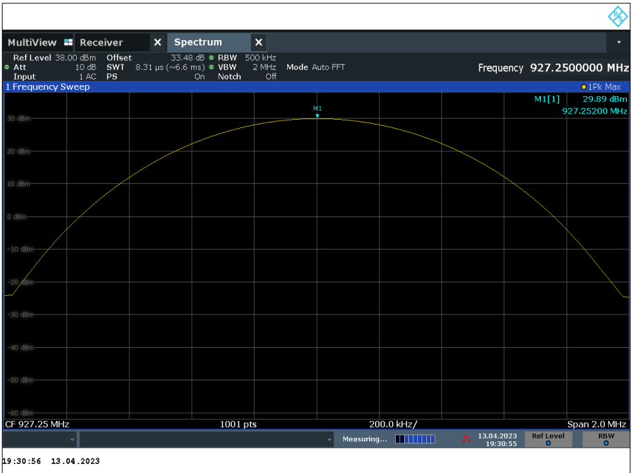
Figure 22 - 927.25
