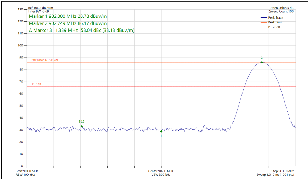
Figure 28 - FHSS, 902.75MHz, Band Edge Frequency 902 MHz
