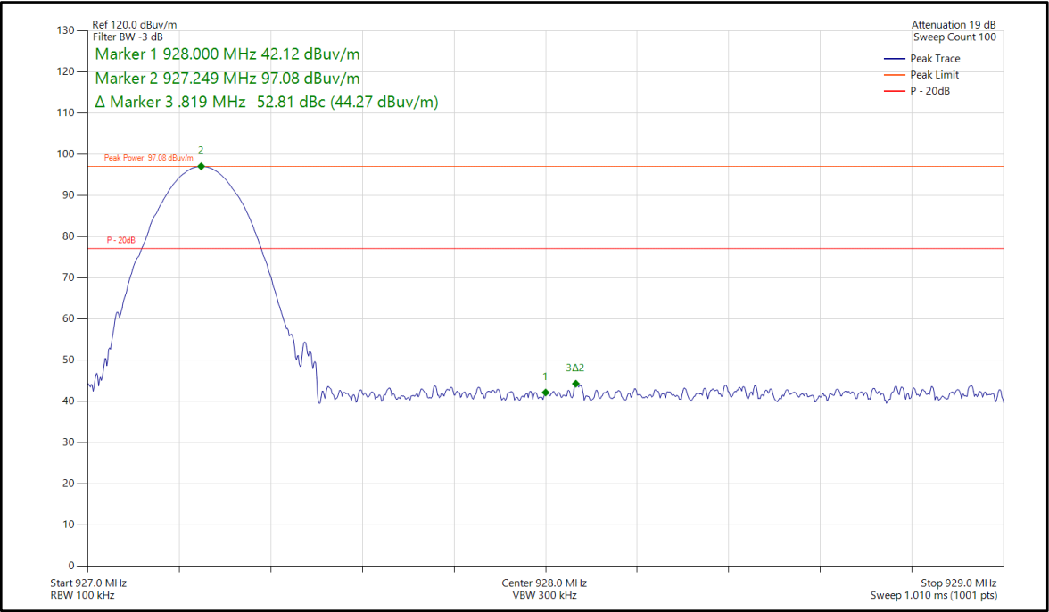
Figure 27 - FHSS, 927.25MHz, Band Edge Frequency 928 MHz
