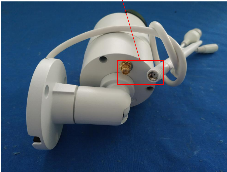
RP-SMA Antenna
