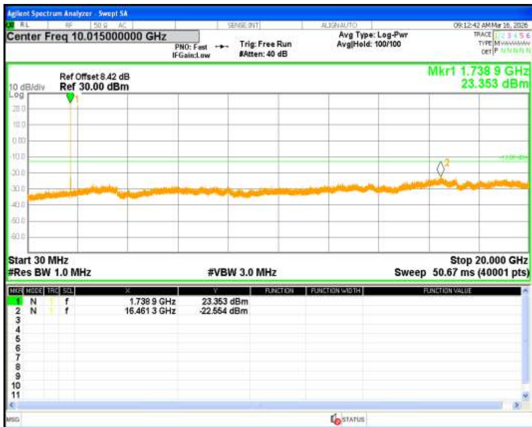
HSDPA Band4 Subtest1 Channel=1513
