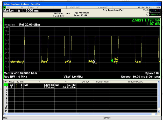
T on1
