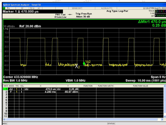
T on2
