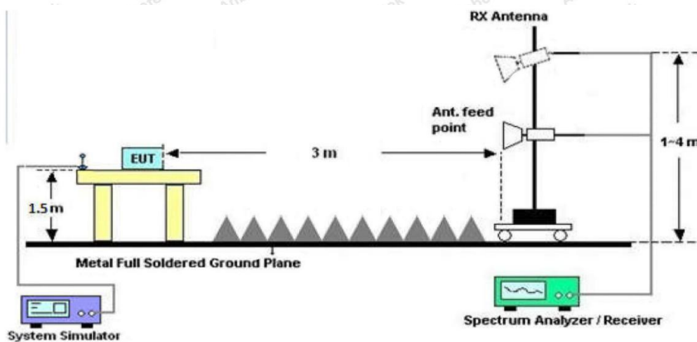
Figure 3. Above 1 GHz
