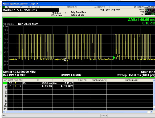
T on2
