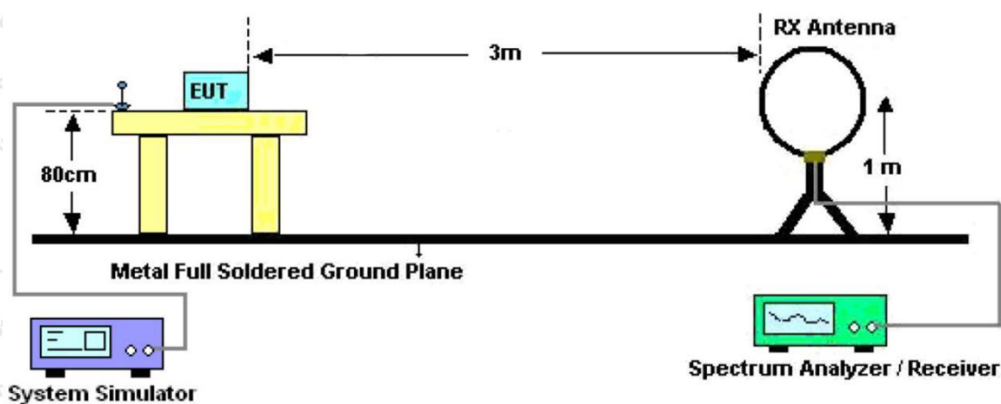
Figure 1. Below 30MHz
