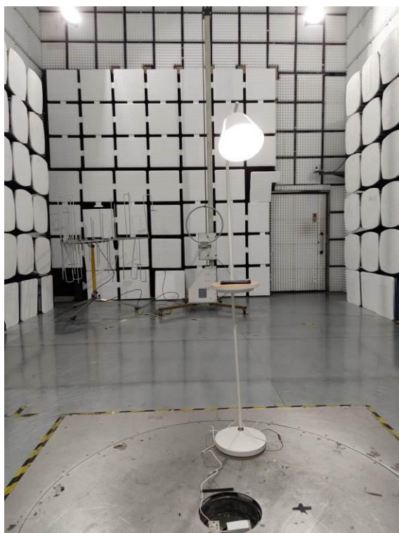
Radiated Emission below 30MHz
