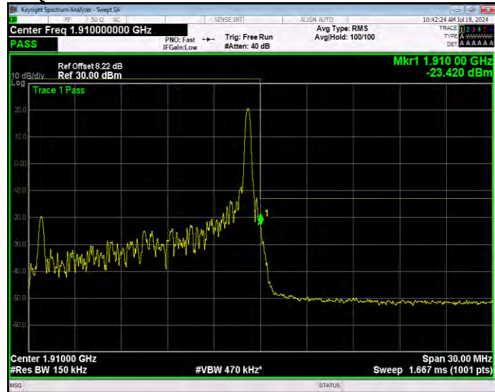
Band2 QPSK BW=15MHz Channel=19125 RB Size=75 Position=#0 Extended
