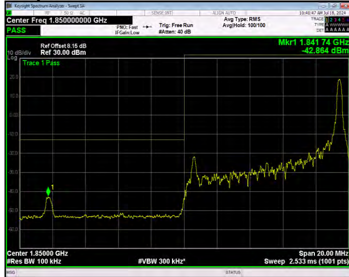
Band2 16QAM BW=10MHz Channel=18650 RB Size=50 Position=#0 Extended
