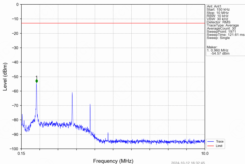
Band2_HSDPA_LCH_1852.4MHz_Subtest 1 NTN
