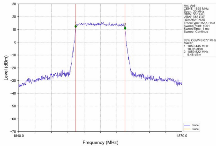
Band25 10MHz 16QAM LCH 1855MHz RB 50 0 NTNV
