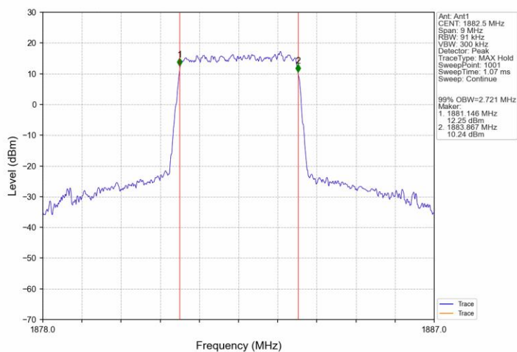
Band25 3MHz QPSK MCH 1882.5MHz RB 15 0 NTNV
