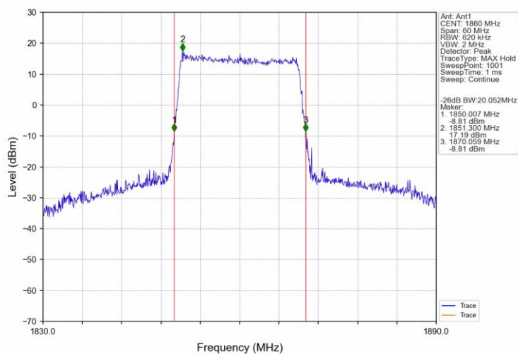
Band25 20MHz 16QAM LCH 1860MHz RB 100 0 NTN
