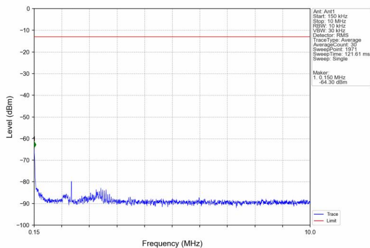
Band66 3MHz QPSK HCH 1778.5MHz RB 1 0 NTV
