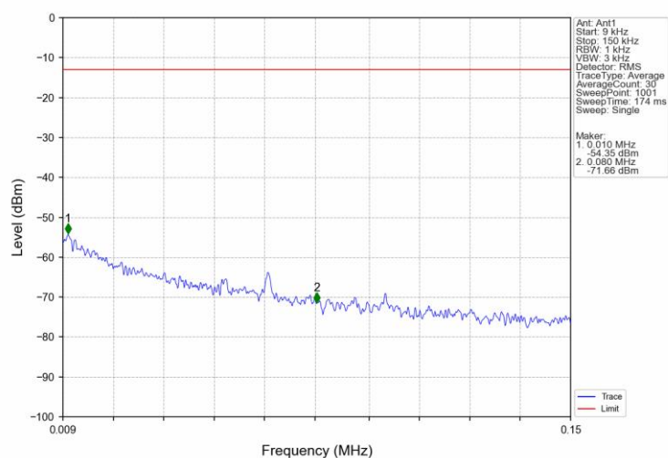
Band66 1.4MHz QPSK HCH 1779.3MHz RB 1 0 NTNV
