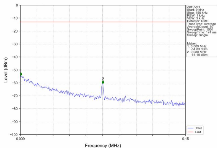
Band66 3MHz QPSK HCH 1778.5MHz RB 1 0 NTV
