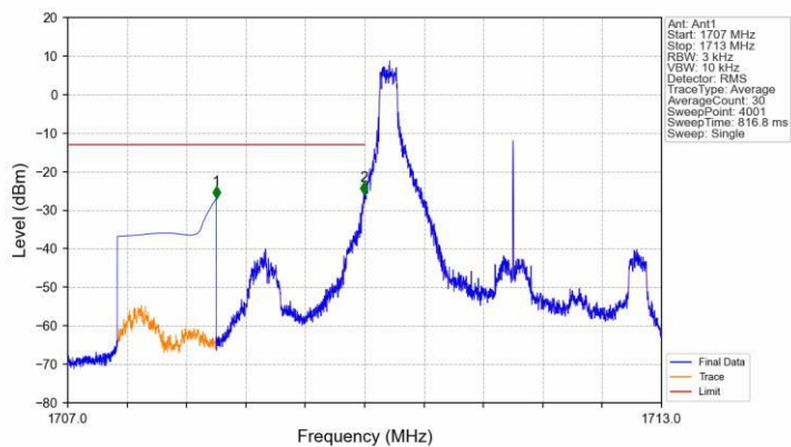
Band66_3MHz_QPSK_LCH_1711.5MHz_RB_1_0_NTNV
