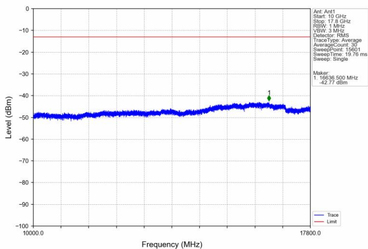
Band66 3MHz 16QAM HCH 1778.5MHz RB 1 0 NTNV
