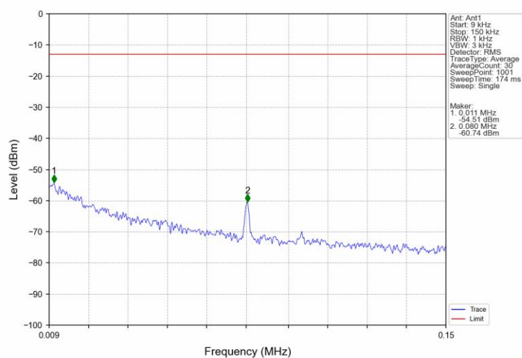
Band66 3MHz 16QAM HCH 1778.5MHz RB 1 0 NTN
