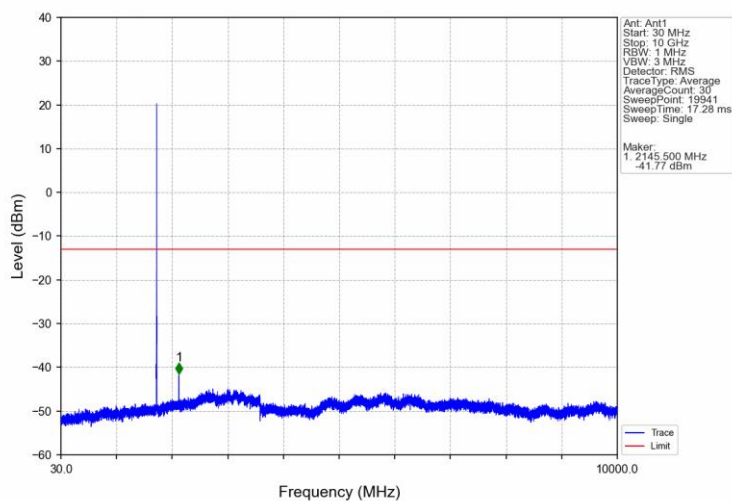
Band66 3MHz 16QAM MCH 1745MHz RB 1 0 NTV
