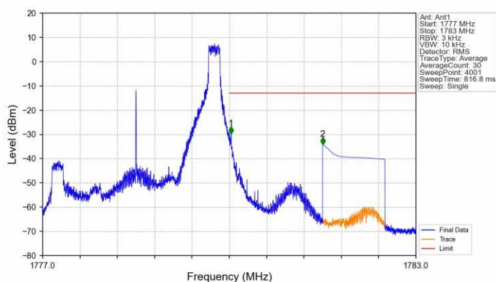
Band66 3MHz QPSK HCH 1778.5MHz RB 1 14 NTV
