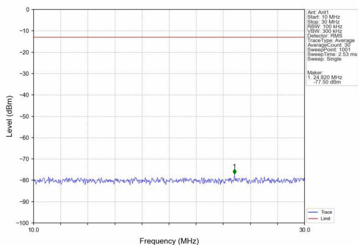
Band66 3MHz 16QAM MCH 1745MHz RB 1 0 NTV
