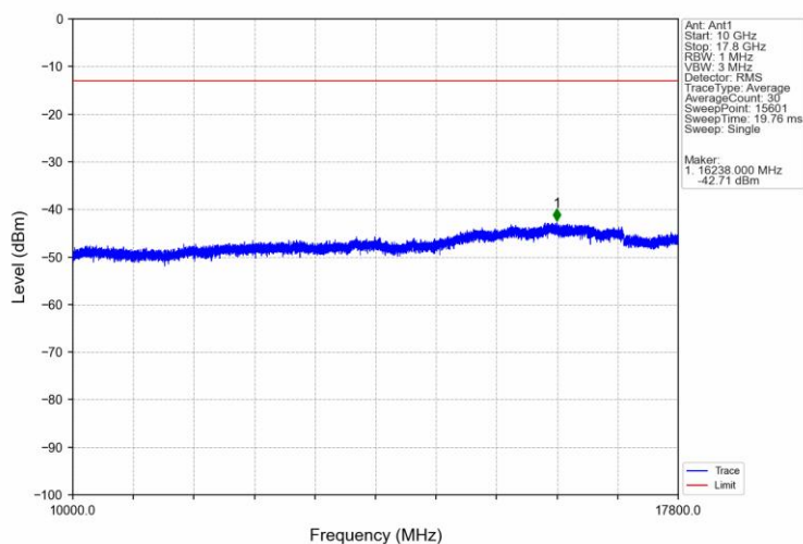
Band66 3MHz QPSK HCH 1778.5MHz RB 1 14 NTV
