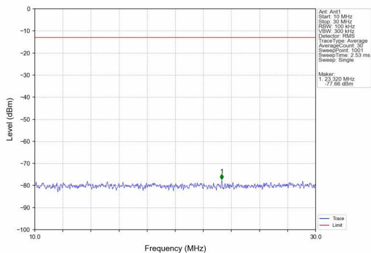
Band66 1.4MHz 16QAM HCH 1779.3MHz RB 1 0 NTN
