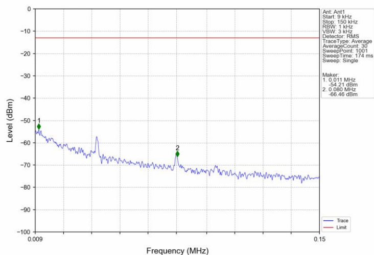
Band66 3MHz 16QAM LCH 1711.5MHz RB 1 0 NTV
