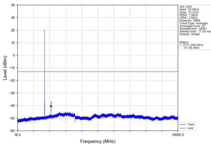
Band66 3MHz 16QAM LCH 1711.5MHz RB 1 0 NTV
