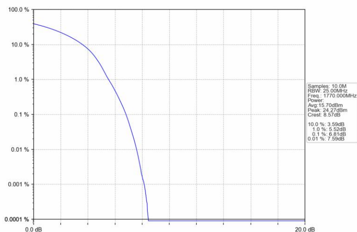
Band66 20MHz 16QAM HCH 1770MHz RB 100 0 NTN
