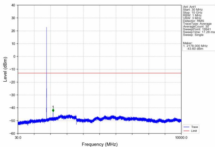
Band66 3MHz QPSK HCH 1778.5MHz RB 1 0 NTV
