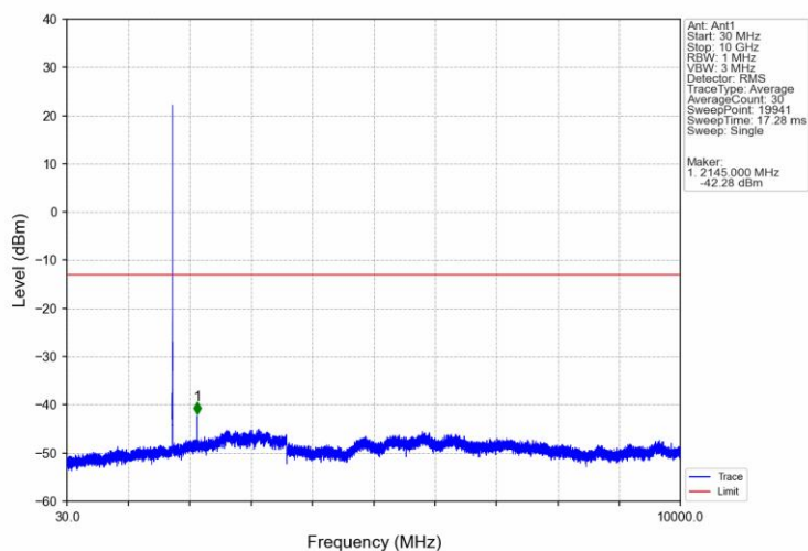
Band66 3MHz QPSK MCH 1745MHz RB 1 0 NTNV
