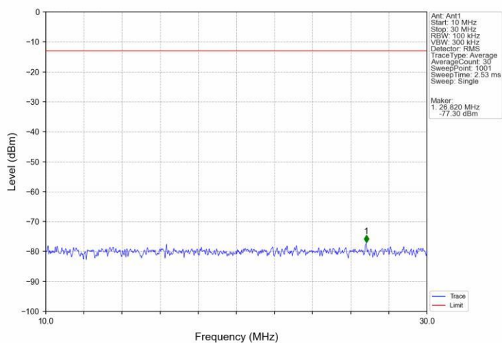
Band66 3MHz 16QAM HCH 1778.5MHz RB 1 0 NTNV
