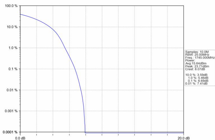
Band66 20MHz 16QAM MCH 1745MHz RB 100 0 NTN
