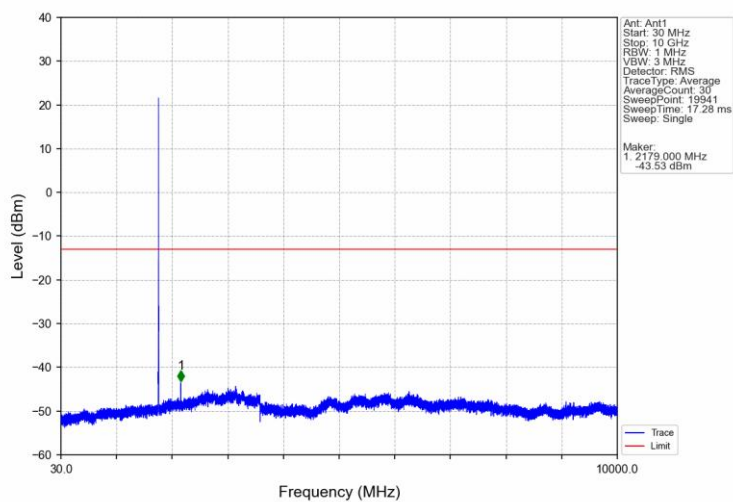
Band66 3MHz 16QAM HCH 1778.5MHz RB 1 0 NTNV
