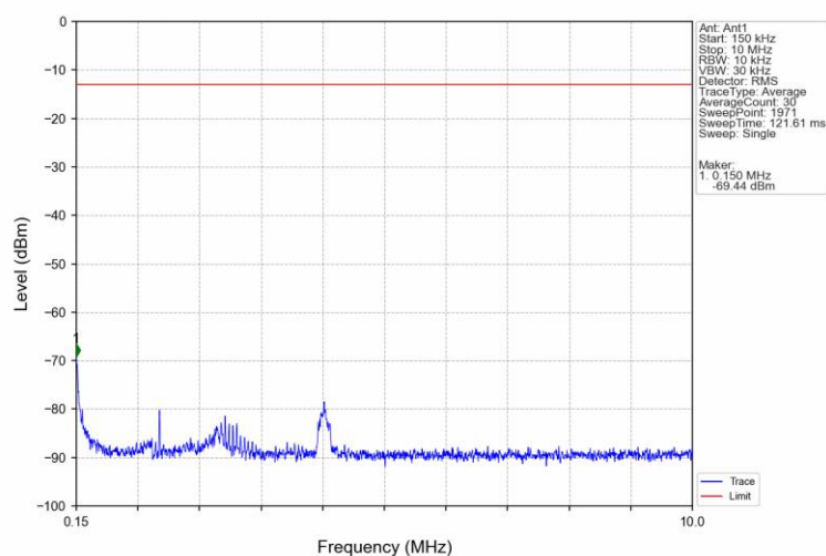
Band66_3MHz_QPSK_LCH_1711.5MHz_RB_1_0_NTNV
