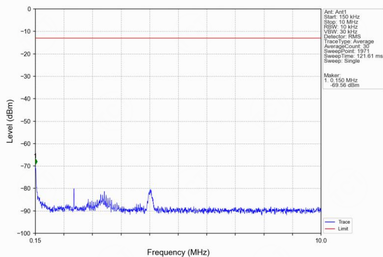
Band66 3MHz 16QAM LCH 1711.5MHz RB 1 0 NTV
