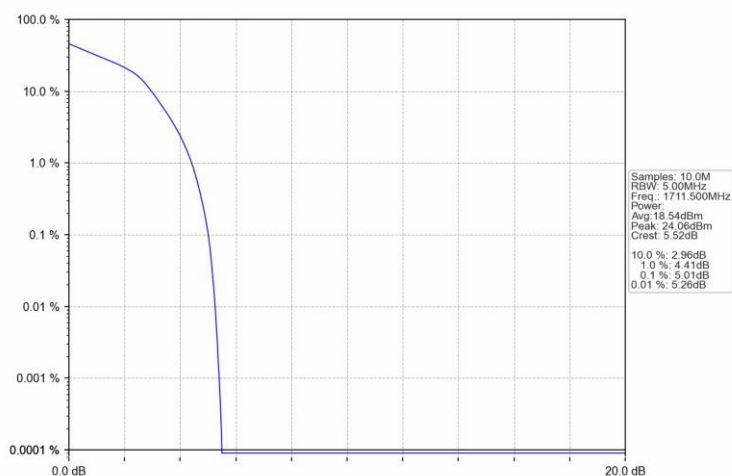
Band66 3MHz 16QAM LCH 1711.5MHz RB 15 0 NTV
