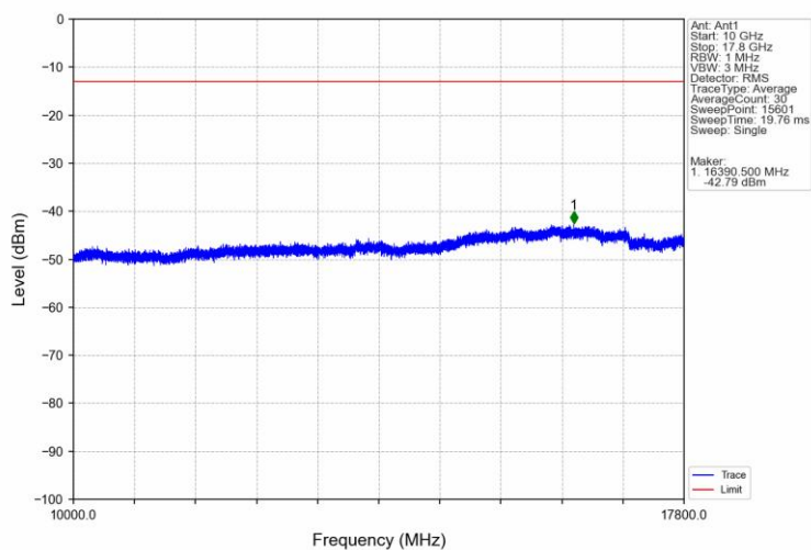
Band66 3MHz QPSK MCH 1745MHz RB 1 0 NTNV
