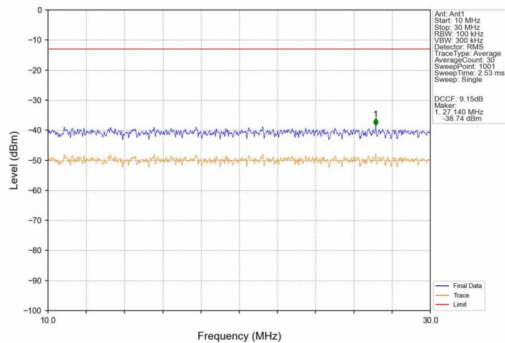
PCS1900_EGPRS_LCH_1850.2MHz_1 TX Slot_NTNV
