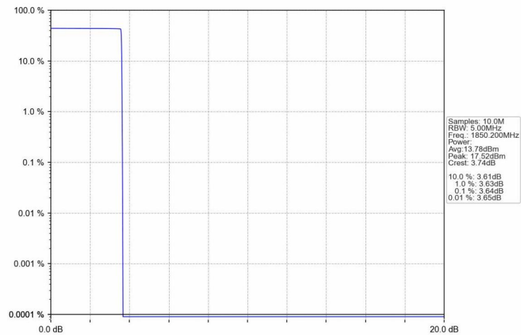
PCS1900_GPRS_LCH_1850.2MHz_4 TX Slots_NTNV
