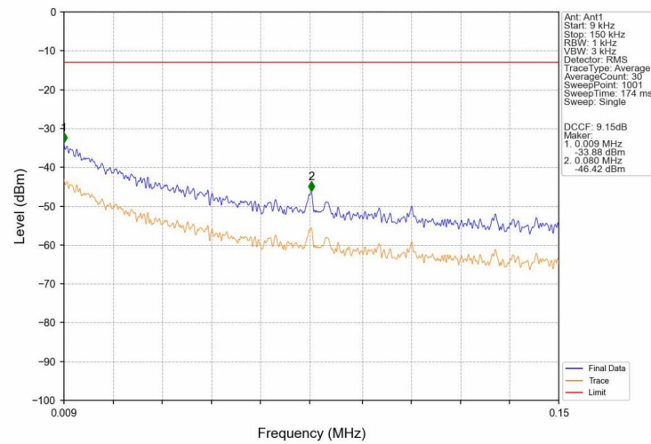
PCS1900_EGPRS_MCH_1880MHz_1 TX Slot_NTNV
