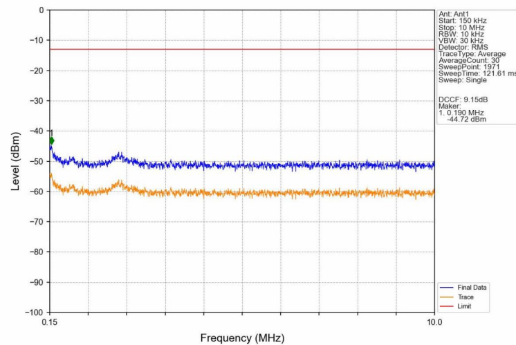
PCS1900_EGPRS_MCH_1880MHz_1 TX Slot_NTNV
